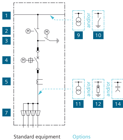
Section feeder panel
