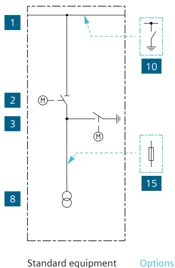
Metering panel
