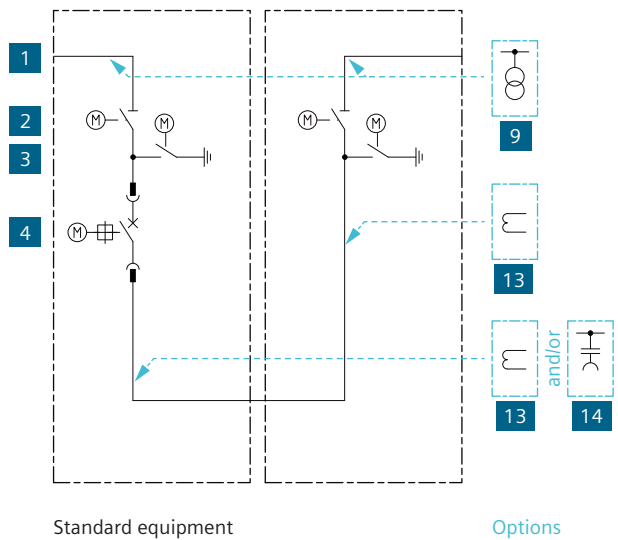
Bus coupler panel
