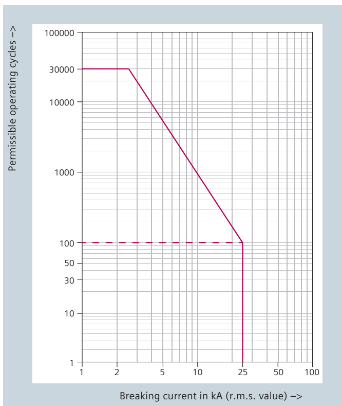
Electrical service life of vacuum interrupter
