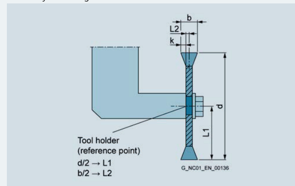
Geometry of slotting saw
