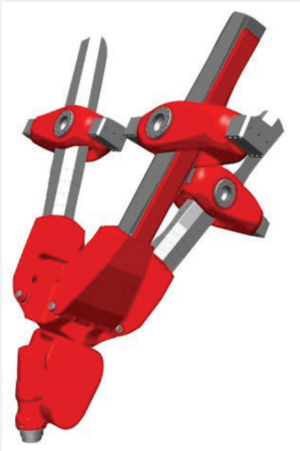
Parallel kinematic type Exechon
