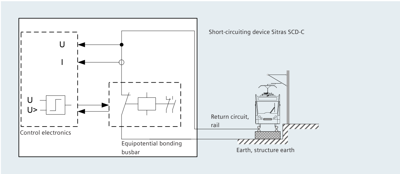
Block diagram of Sitras SCD-C
