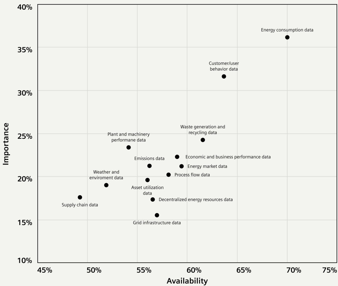
Data type importance by availability (both in the context of improving decarbonization and resource efficiency in operations)
