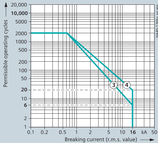
Rated short-circuit breaking current 16 kA
