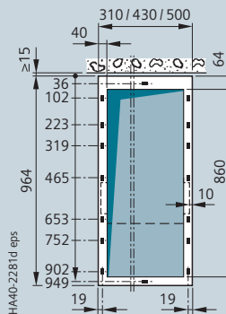
With base extension (floor opening depending on selected cable connection/arrester) Deeper by 105 mm
