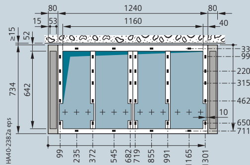
Panel block RRT-RRT Compact
