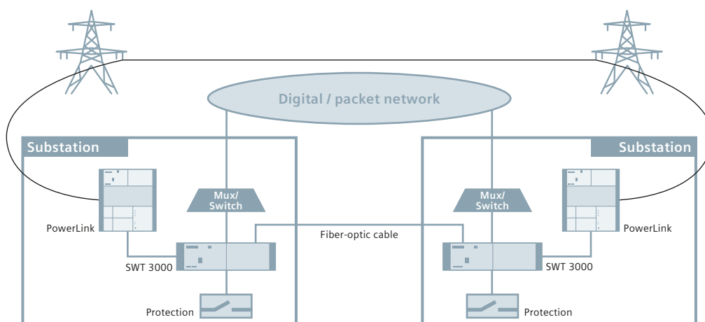
SWT 3000 – transmission routes
