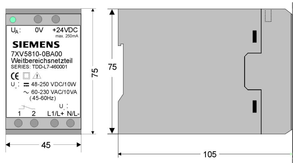
Abb. 4: Dimension Drawings
