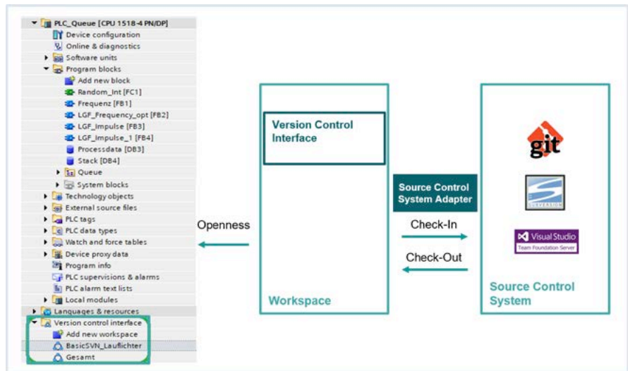
Connection of versioning systems to the TIA Portal with the Version Control Interface (VCI)
