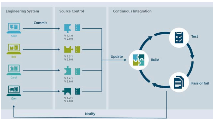
Basic principle of software development with Continuous Integration
