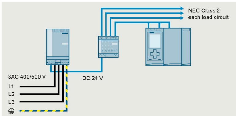
Several NEC Class 2 control circuits each supplied via a separate output of an NEC Class 2 selectivity module
