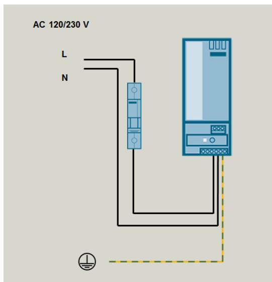
Primary connection of a single-phase power supply without grounding the N conductor.
