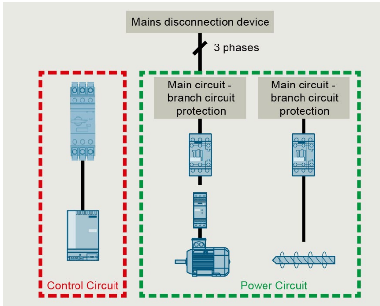
Connection of a three-phase power supply.
