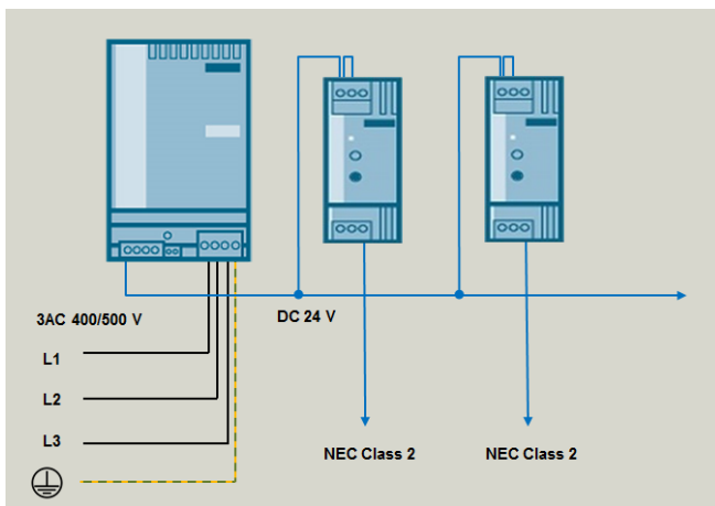
NEC Class 2 control circuits each supply from a central power supply via an NEC Class 2 redundancy module (without redundancy)
