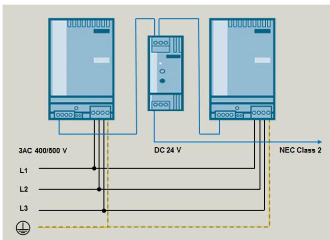
A redundant NEC Class 2 control circuit supplies power from two power supplies via an NEC Class 2 redundancy module
