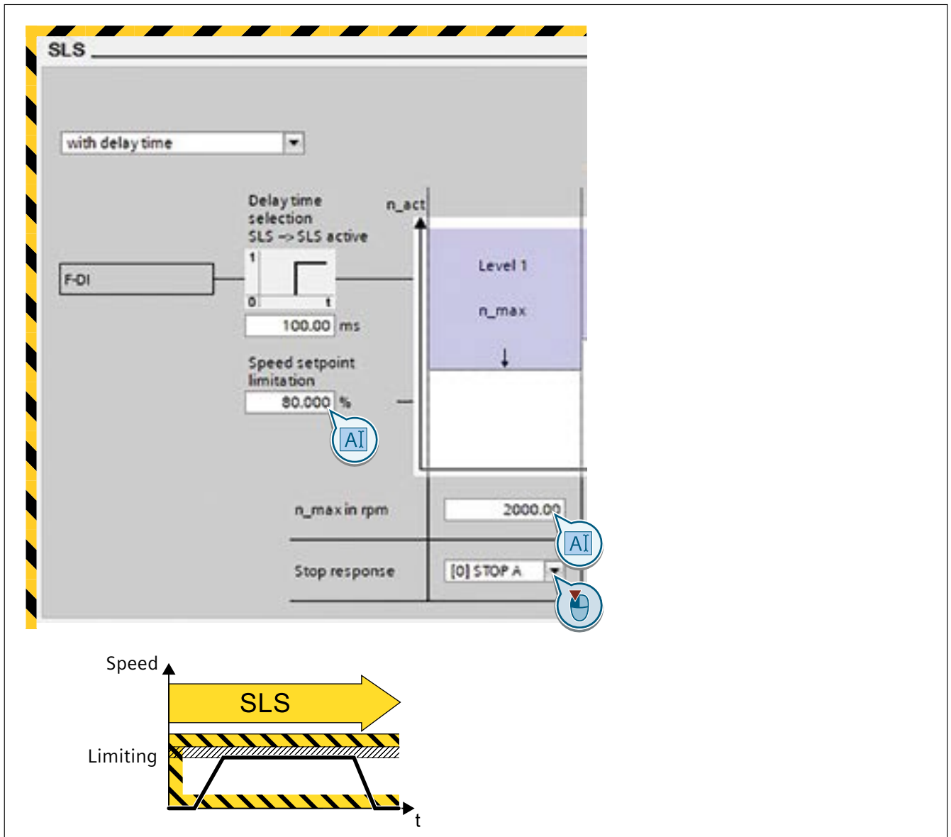
Figure 2-14 Monitoring, limiting and stop response of the SLS function
