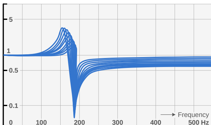
Attenuation of harmonic voltages of a compensation system with 7 % choking in case of different capacitor modules (levels).
