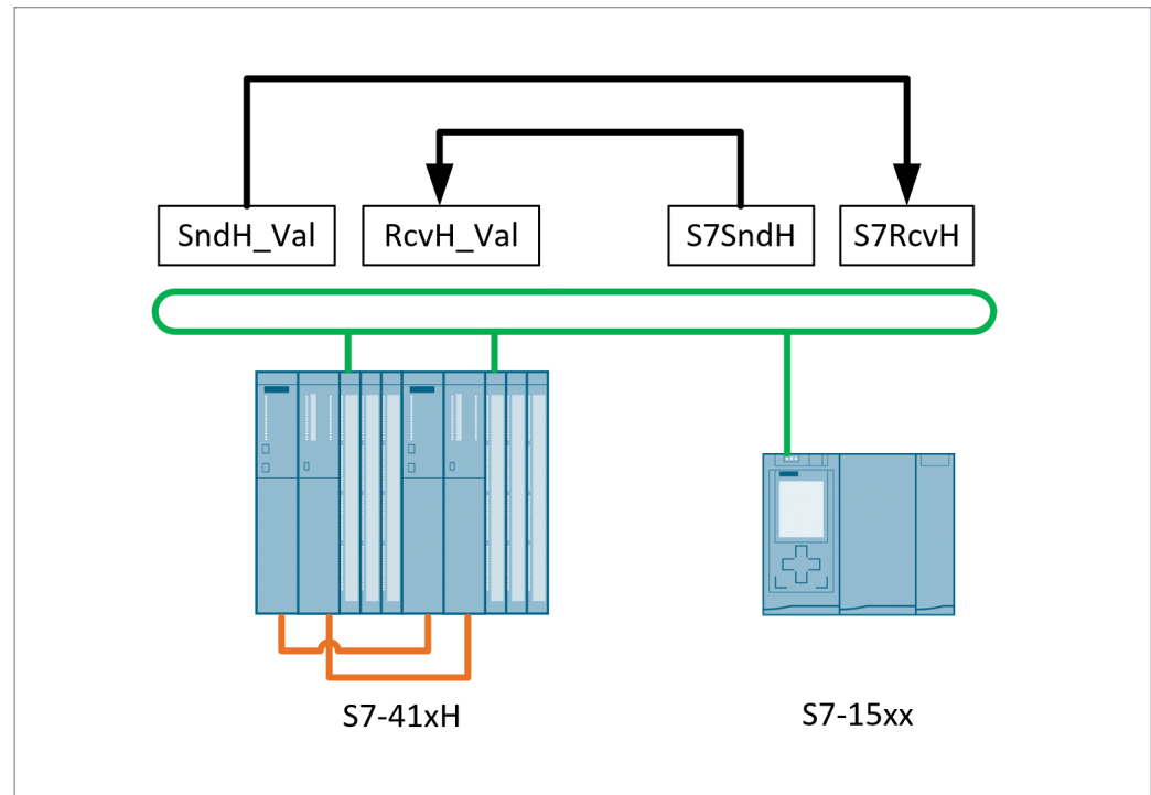
The Industry Library enables communication between SIMATIC S7-400 controllers and S7-1500 PLCs, giving operators the option to run an entire plant from a single SIMATIC PCS 7 operator station.
