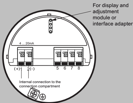
SITRANS LG series connections
