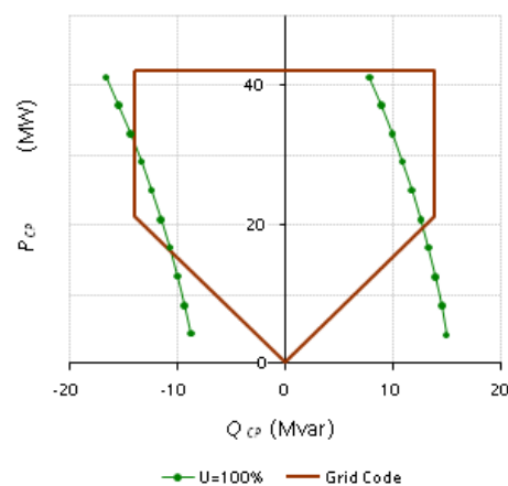
Figure 1: Example of reactive power capability curves
