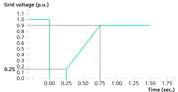
Figure 2: Example of a fault ride-through requirement curve
