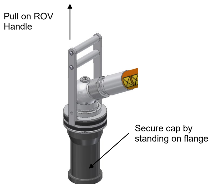
Figure 6 - ROV Plug Cap
