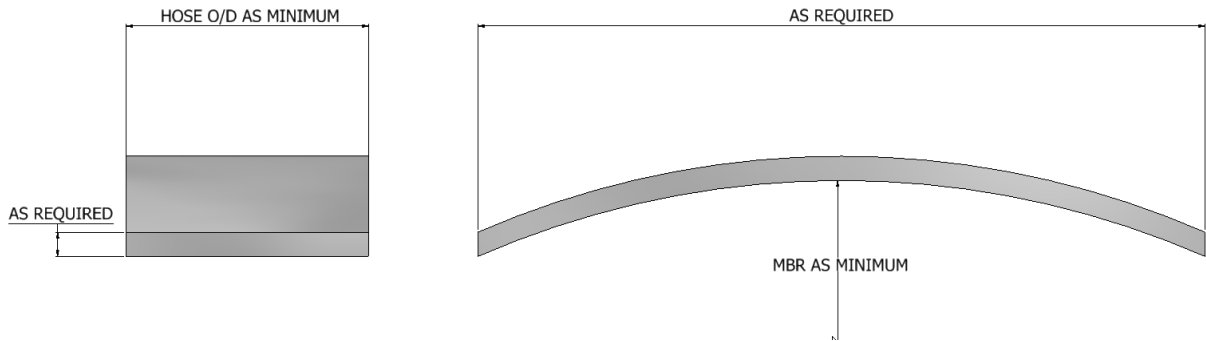
Figure 23- Plate Former
