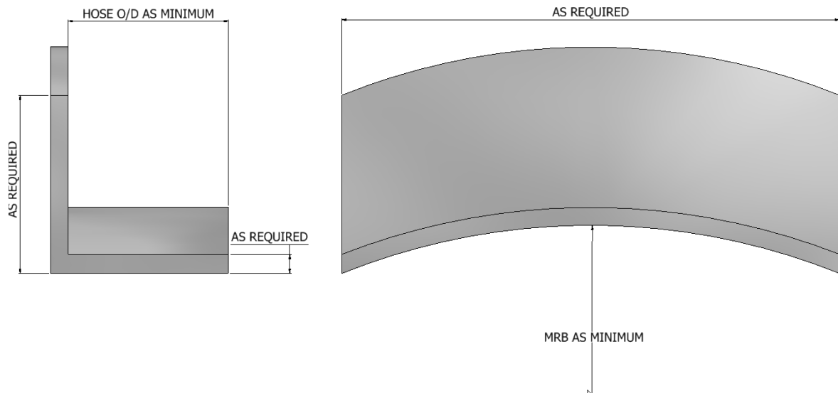
Figure 25- 'L' Former
