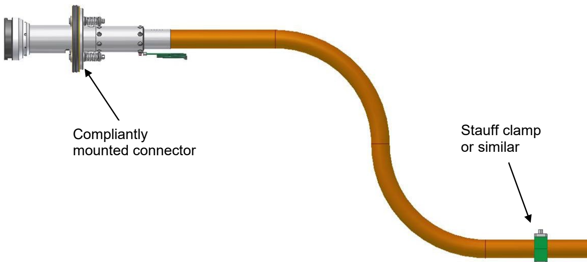
Figure 27 – Potential clamping of hose on compliant connector
