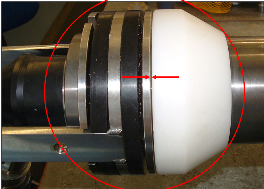
Figure 11 – Type 1 Mating check - Connectors fully mated. Note small gap between flanges.
