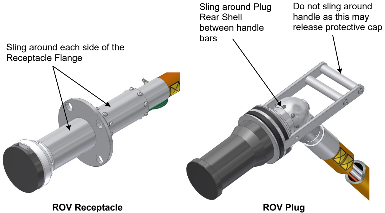
Figure 4 - Recommended lift positions – Plug & Receptacle
