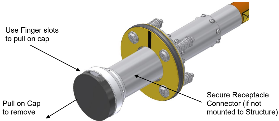
Figure 7 - ROV Receptacle Cap
