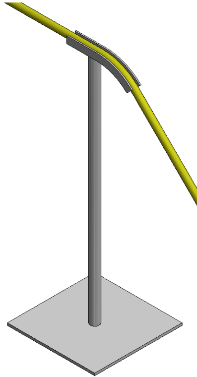
Figure 30- fabricated stand with former used for hose support
