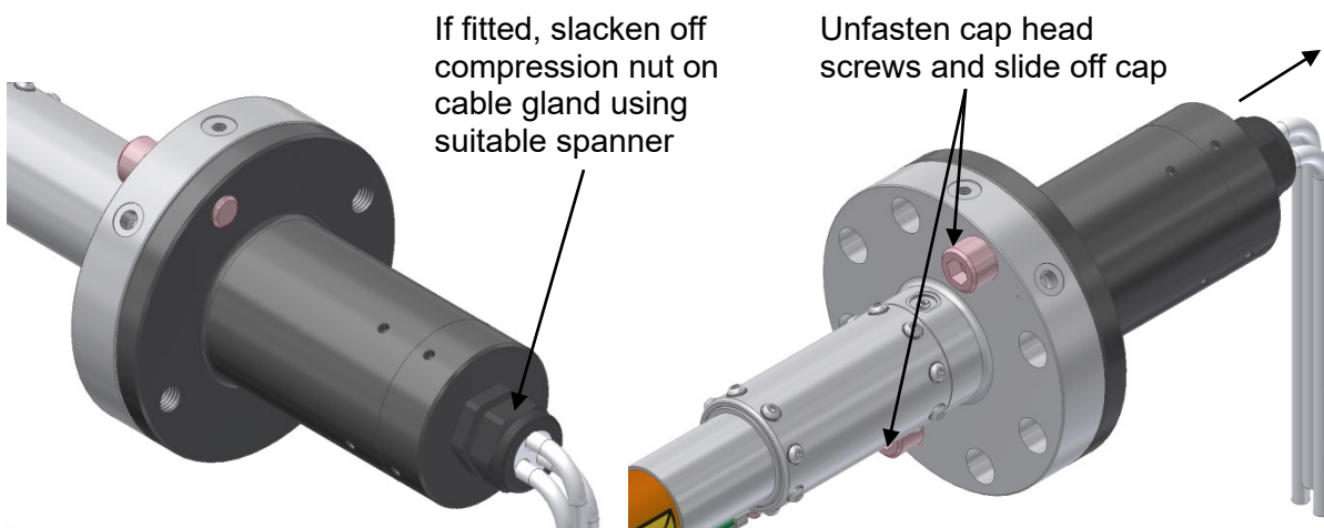
Figure 8 - Penetrator Cap
