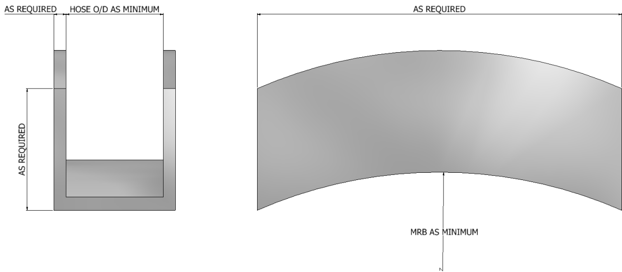
Figure 24- 'U' Former
