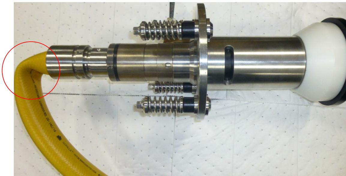
Figure 22-Hose kink due to acute angle and weight application
