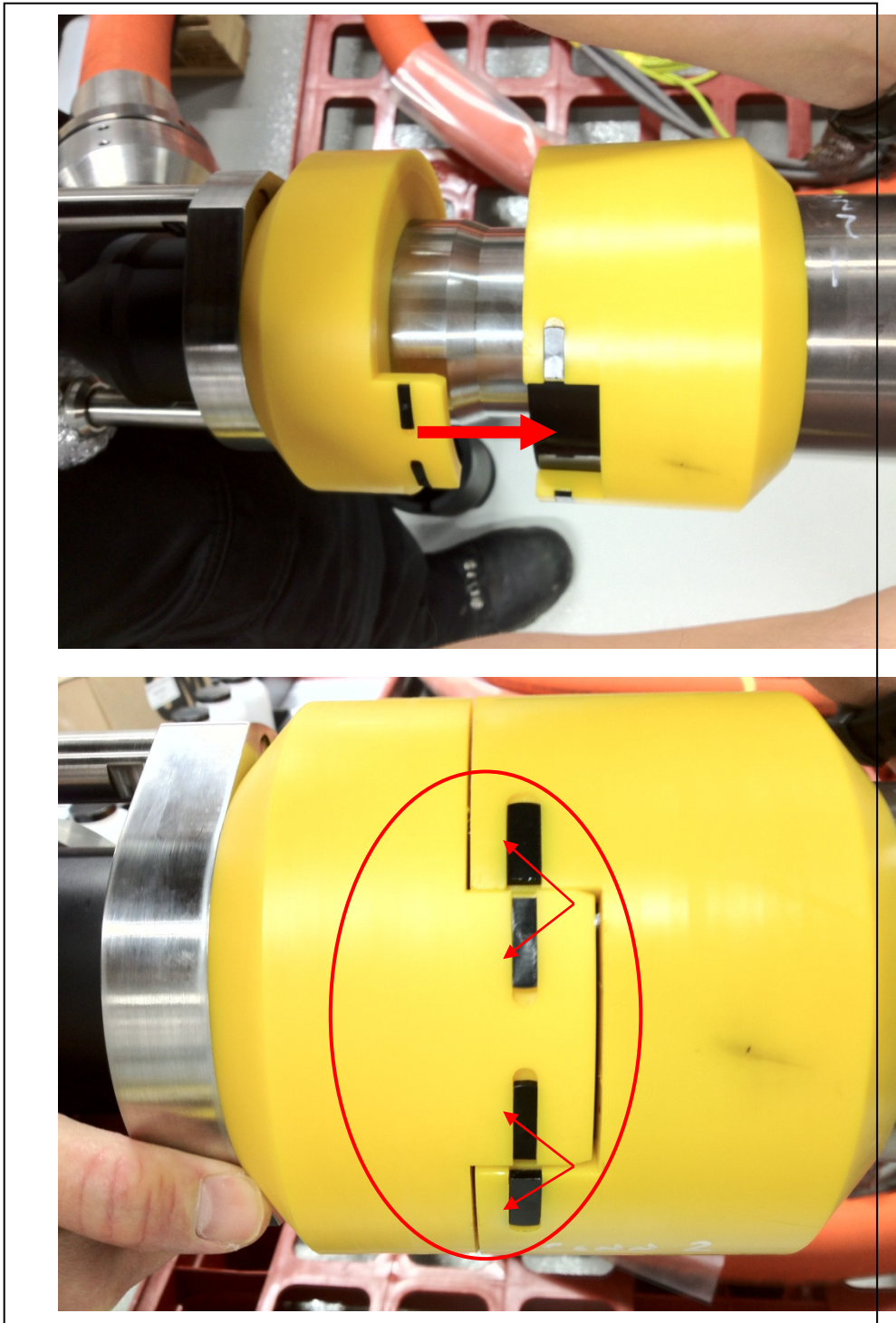
Figure 12 – Type 2 Mating check - Connectors fully mated. Note alignment of black markers on Plug & Receptacle. The thinner marker of the Plug should fall within the wider marker on the Receptacle Cone.
