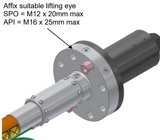
Figure 4 - Recommended lift positions – Plug & Receptacle
