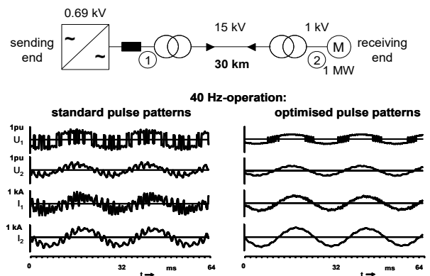
Figure 4: Electrical circuit and voltage and current at the sending end ( U_1 , I_1 ) and receiving end ( U_2 , I_2 ) of the converter configuration with and without optimized pulse patterns
