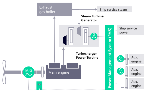
Figure 2: Generation concept for a container vessel
