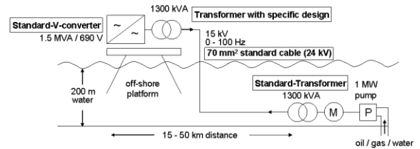
Figure 3: Configuration of a multi-phase underwater booster station
