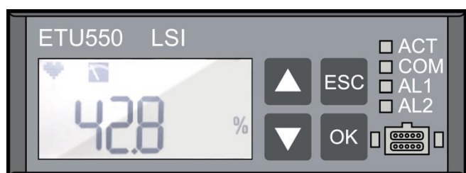
Representation of the health indicator (in %) on the display of the Electronic Trip Unit ETU
