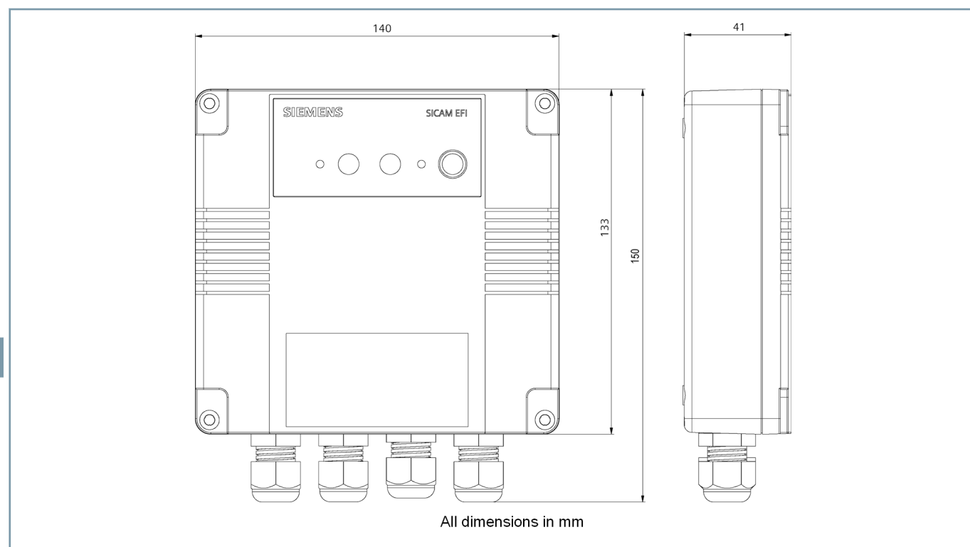
Figure 3.3/1 SICAM EFI Front View and Side View
