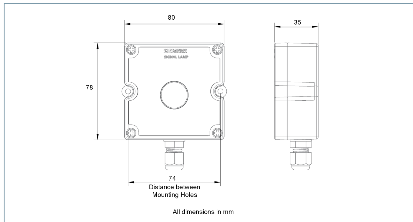
Figure 3.3/2 Siemens Signal Lamp Front and Side View
