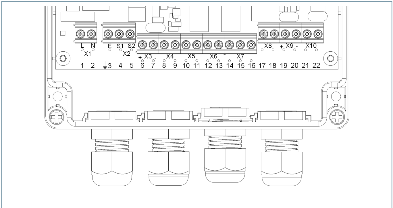
Figure 3.4/1 SICAM EFI Terminal Details
