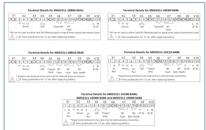
Figure 3.4/2 Terminal Details for SICAM EFI Variants
