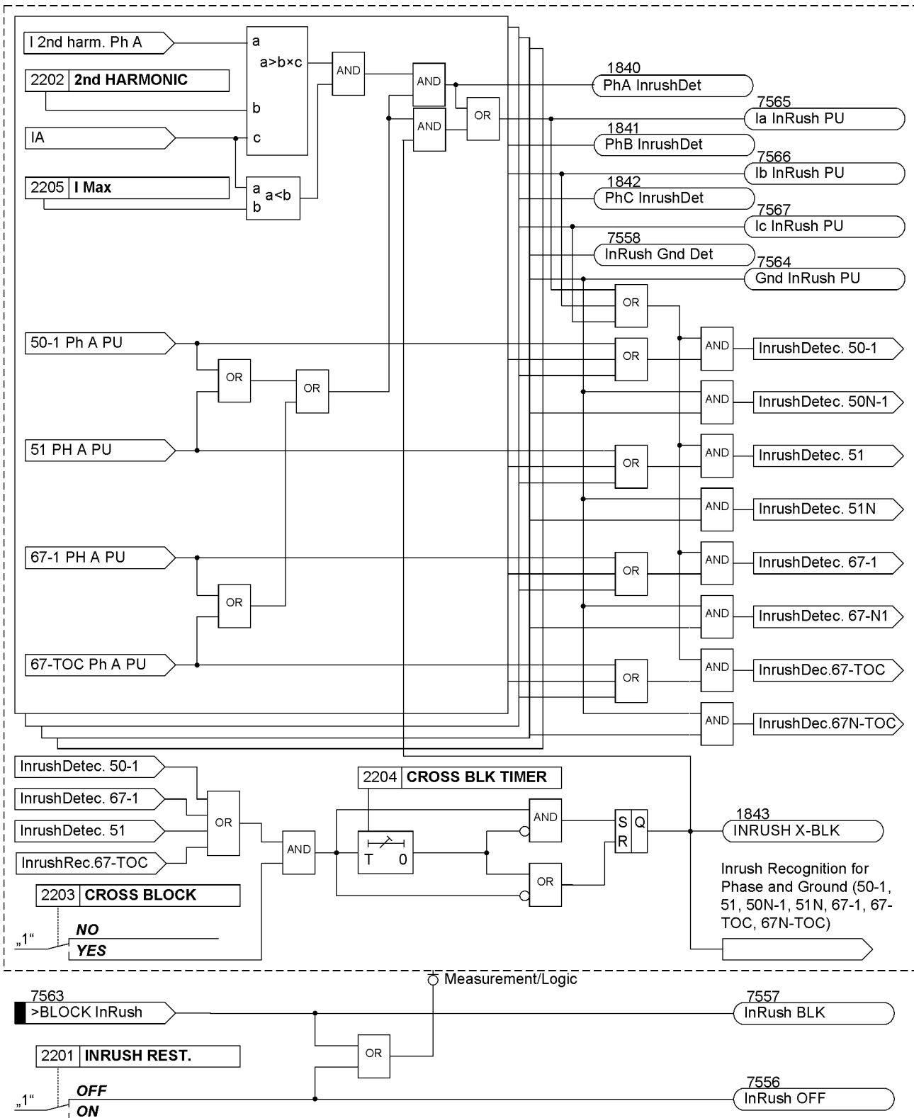
Figure 2-19 Logic diagram for inrush restraint
