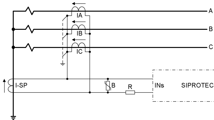
Figure 2-45 Connection scheme of the ground fault differential protection according to the high impedance principle
