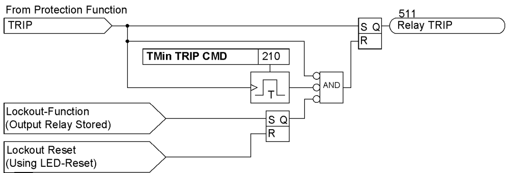
Figure 2-130 Terminating the Trip Signal
