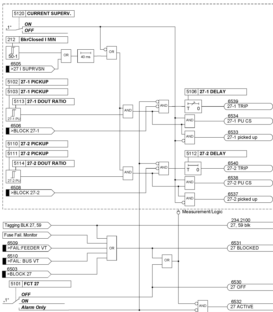
Figure 2-49 Logic diagram of the undervoltage protection
