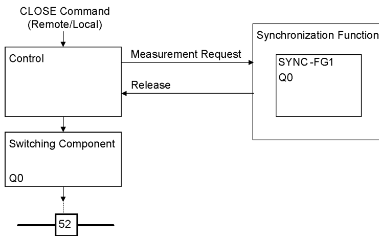
Figure 2-123 Interaction of control and synchrocheck function
