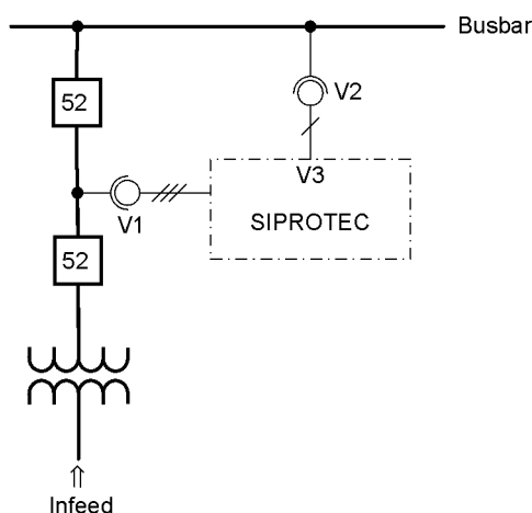
Figure 3-26 Measuring voltages for synchrocheck
