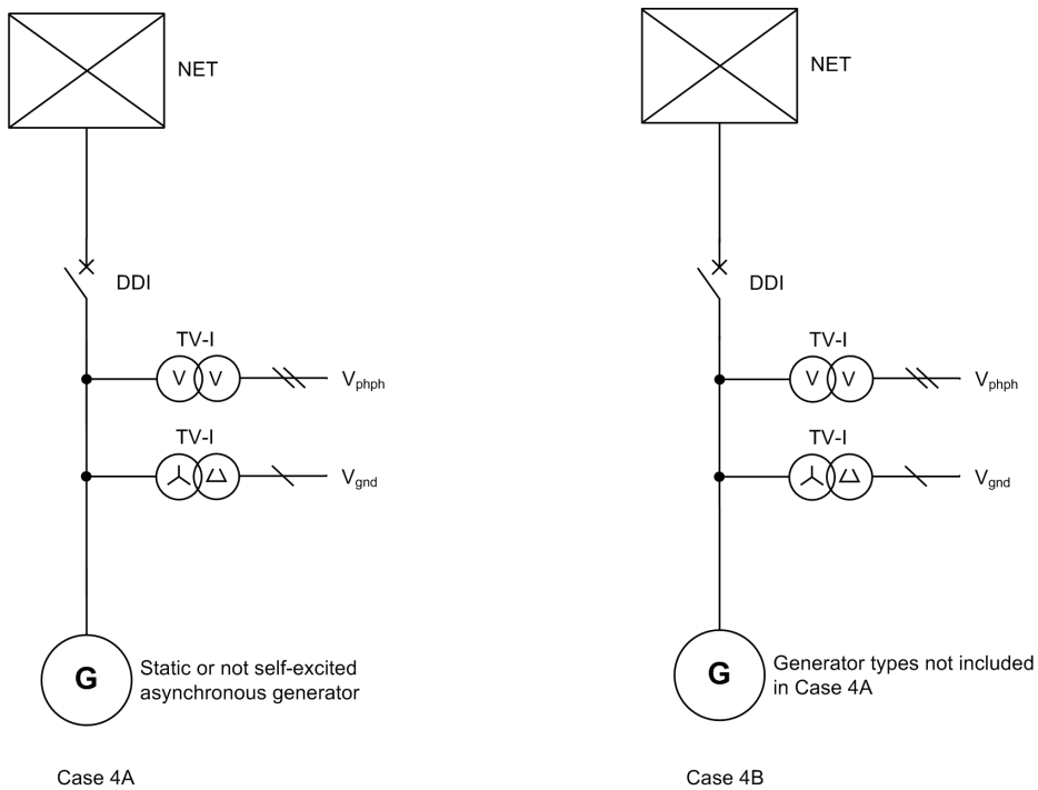
Figure 2-53 Application guide of VT installation position: Case 4
