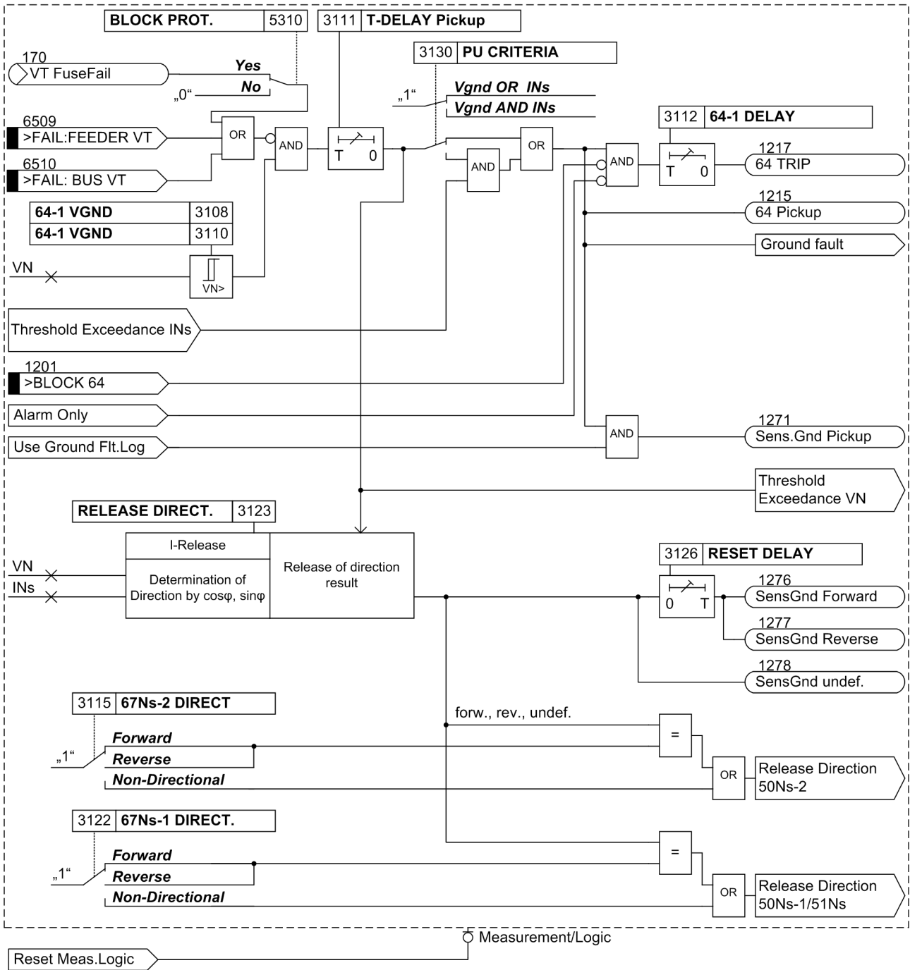
Figure 2-85 Logic diagram of the V_{N>} element for \cos-\varphi / \sin-\varphi measurement
