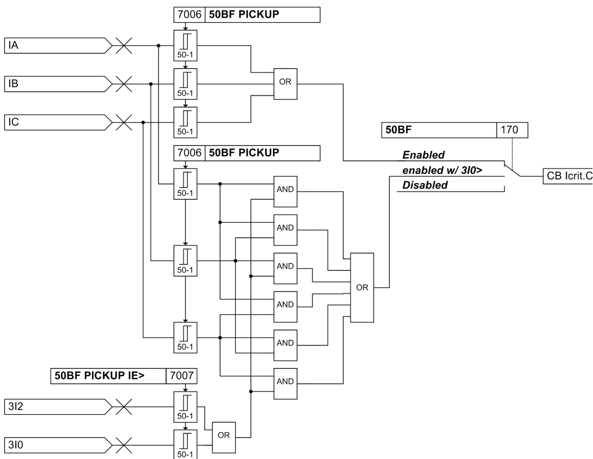
Figure 2-107 Monitoring of the current flow
