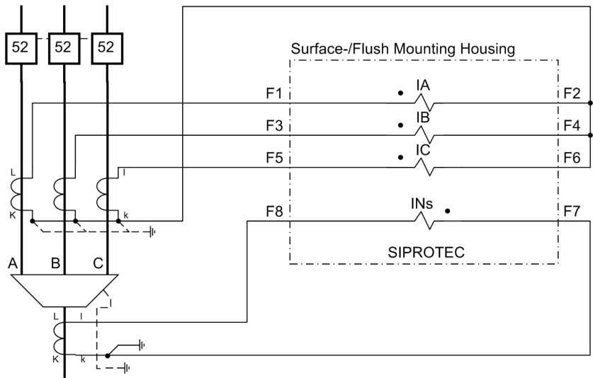
Figure A-11 Current transformer connections to three current transformers - ground current from additional cable-type current transformer for sensitive ground fault detection
