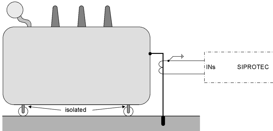
Figure 2-43 Tank protection principle
