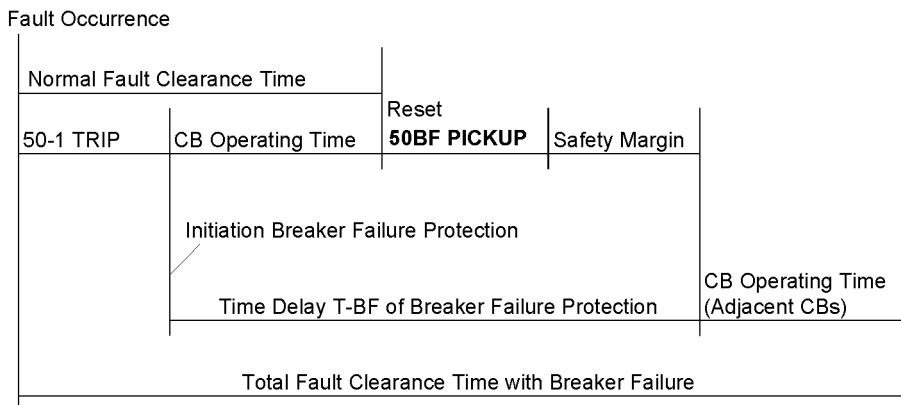
Figure 2-110 Time sequence example for normal clearance of a fault, and with circuit breaker failure
