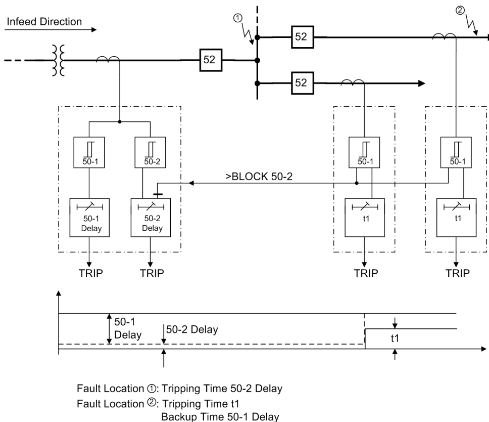
Figure 2-20 Reverse interlocking protection scheme
