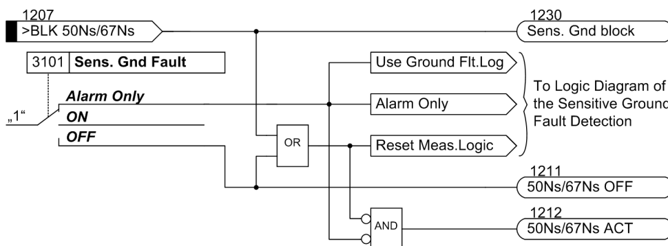
Figure 2-84 Activation of the sensitive ground-fault detection for \cos\varphi / -\sin\varphi measurement
