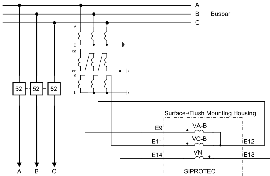
Figure A-22 Voltage transformer connections to two voltage transformers (phase-to-phase voltages) and broken delta winding (da-dn) – appropriate for all networks
