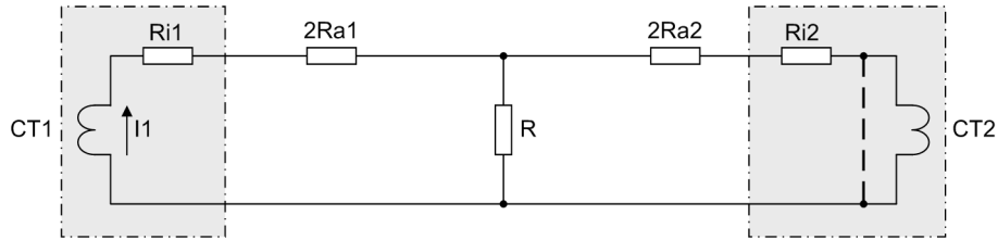
Figure 2-44 Simplified equivalent circuit of a circulating current system for high-impedance protection
