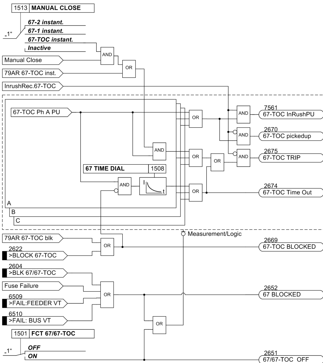
Figure 2-27 Logic diagram for the directional overcurrent protection: 67-TOC relay element
