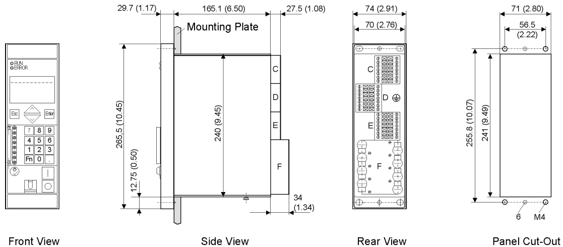
Figure 4-11 Dimensional drawing of a 7SJ80 for panel flush or cubicle mounting (housing size \frac{1}{6} )
