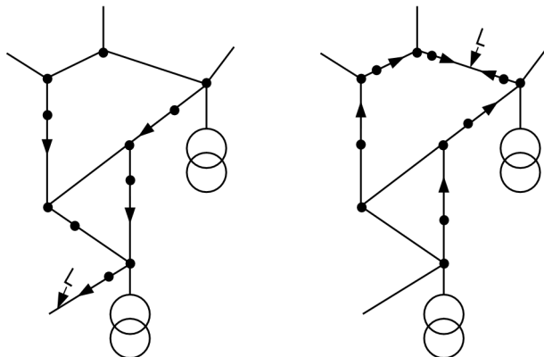
Figure 2-93 Determination of the ground fault location based on directional indicators in the meshed system
