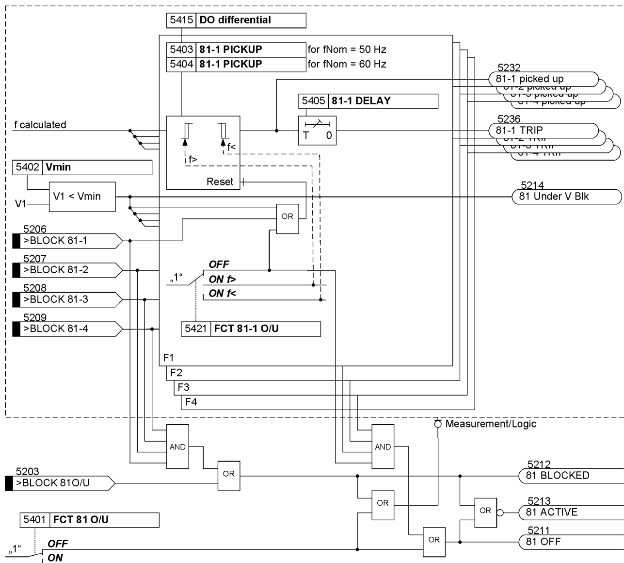
Figure 2-62 Logic diagram of the frequency protection
