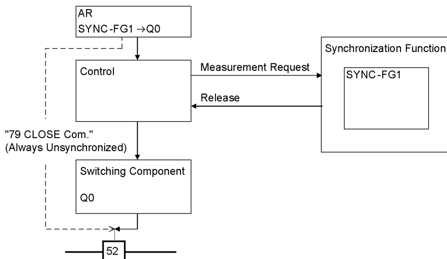
Figure 2-124 Connection of the automatic reclosing function to the synchrocheck function
