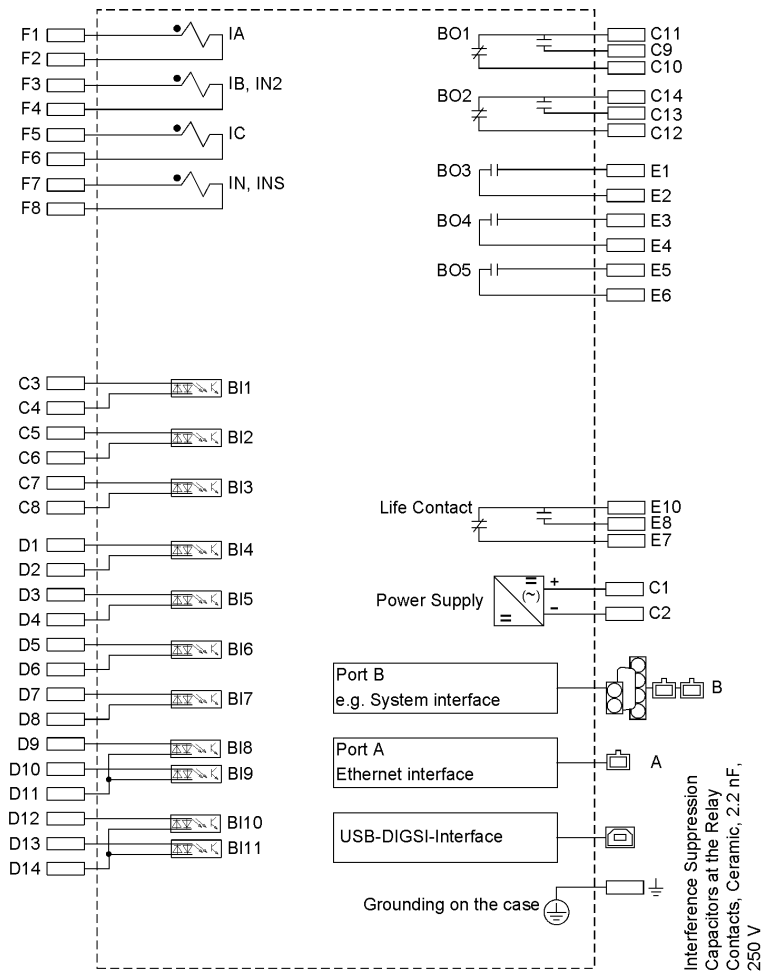
Figure A-5 Connection diagram 7SJ807*
