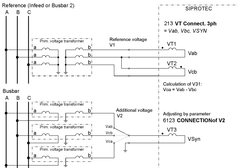
Figure 2-127 Phase-to-phase voltage connection (open-delta connection)
