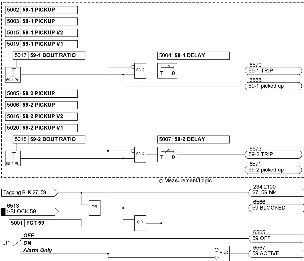
Figure 2-46 Logic diagram of the overvoltage protection
