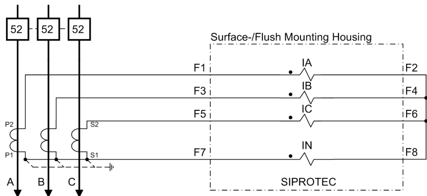
Figure A-7 Current transformer connections to three current transformers and neutral point current (ground current) (Holmgreen connection) – appropriate for all networks
