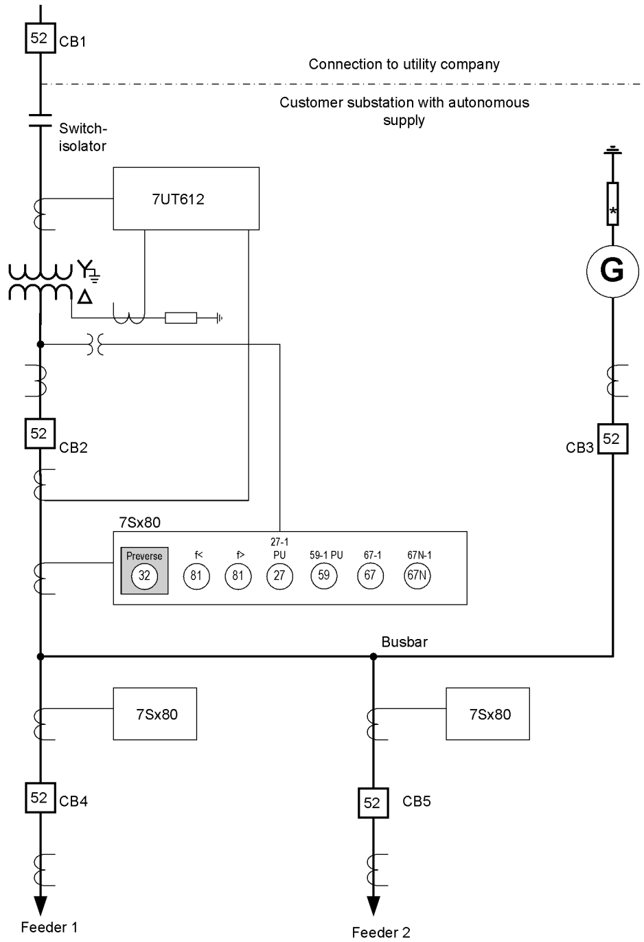
Figure 2-112 Example of a substation with generator self-supply
