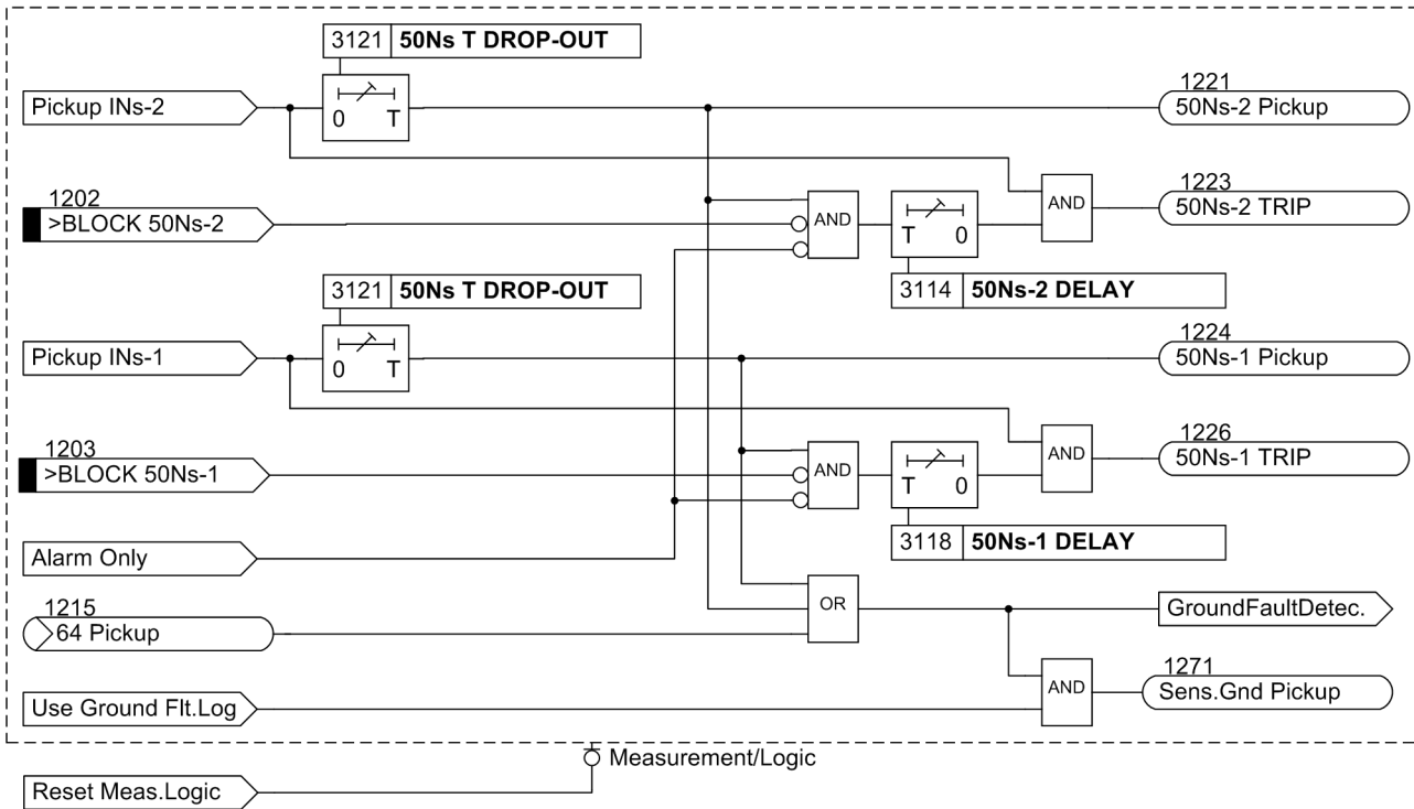
Figure 2-91 Logic diagram for U0-/I0 -φ measurement, part 2
