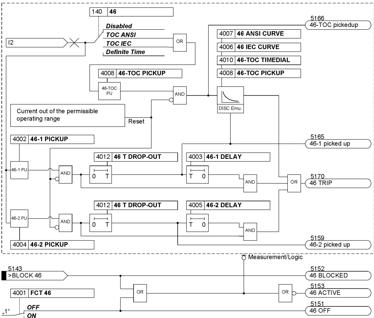
Figure 2-61 Logic diagram of the unbalanced load protection
