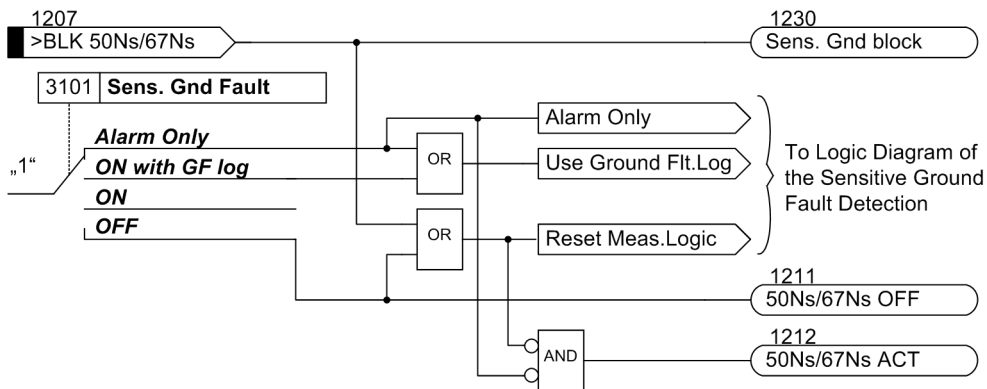
Figure 2-89 Activation of the sensitive ground fault detection for V_0/I_0-\varphi measurement
