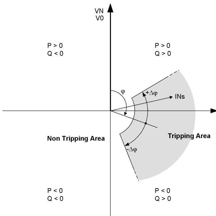
Figure 2-88 Tripping range of V_0/I_0-\varphi characteristic
