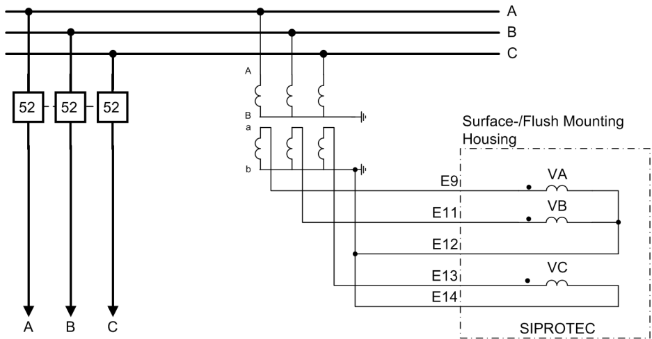
Figure A-23 Example for connection type "VAN, VBN, VCN" busbar-side voltage connection
