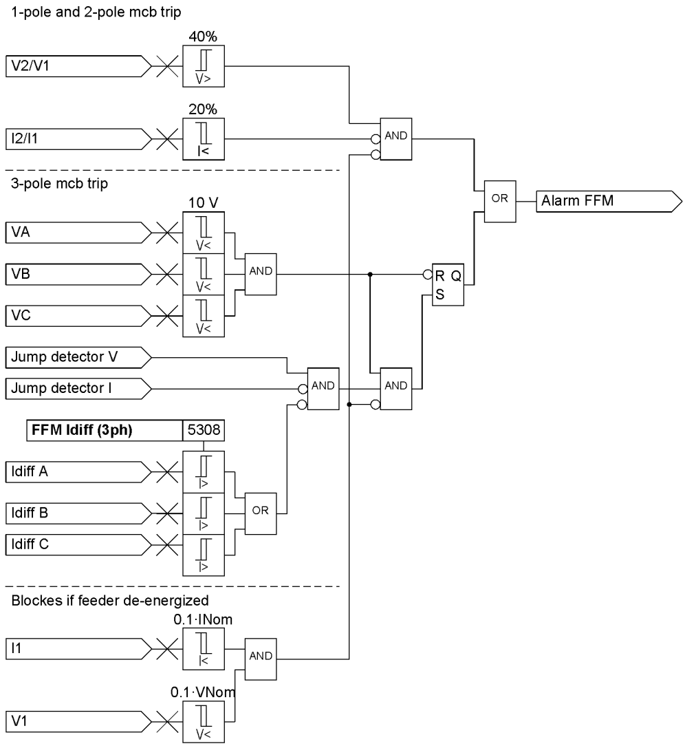
Figure 2-74 Logic diagram of the Fuse Failure Monitor for isolated systems
