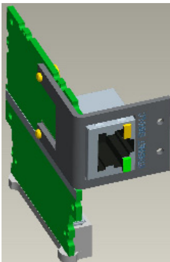
Figure 3-7 Ethernet interface with support frame
