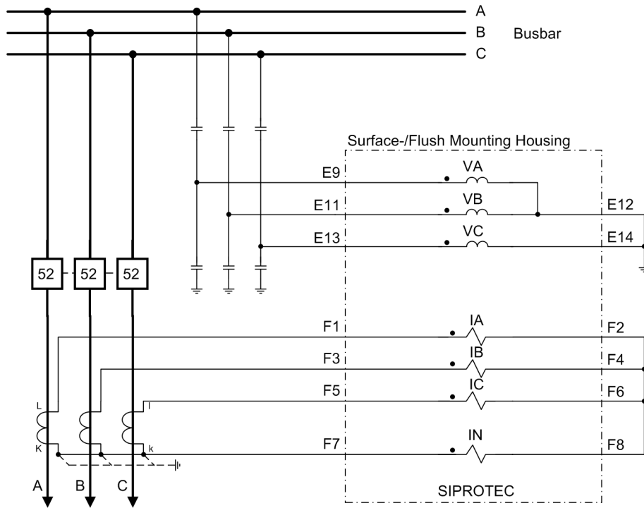
Figure A-13 Transformer connections to three current transformers and three voltage transformers - capacitive -
