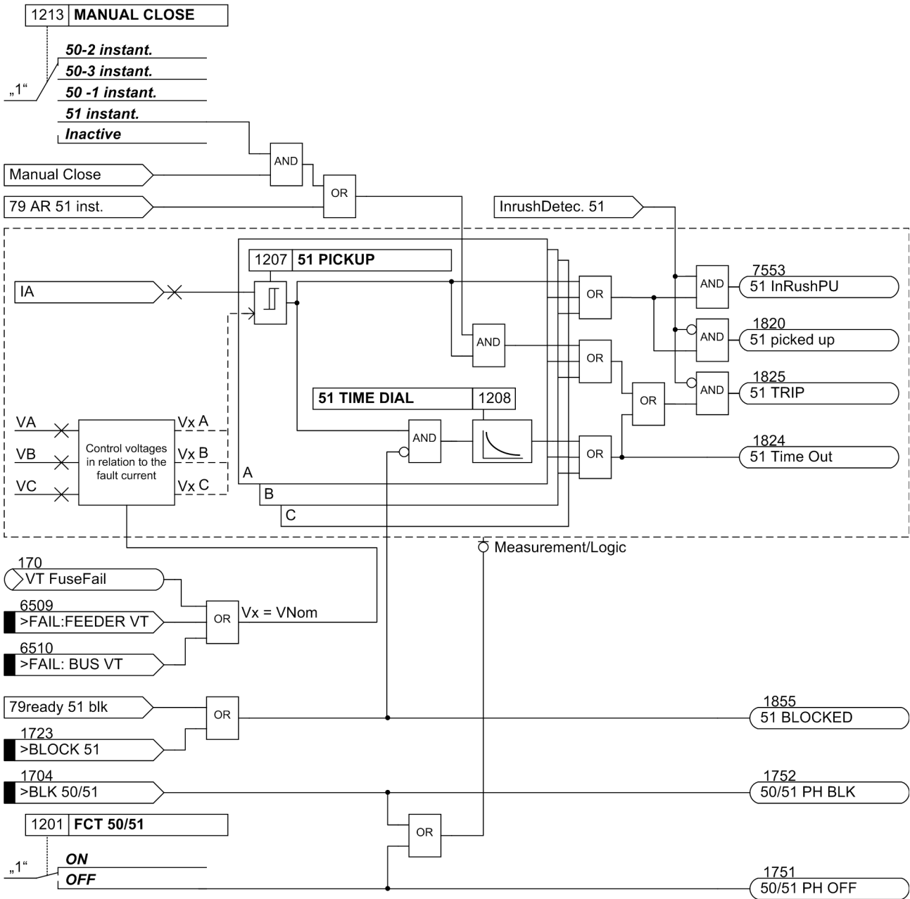
Figure 2-18 Logic diagram of the voltage-restraint inverse-time overcurrent protection
