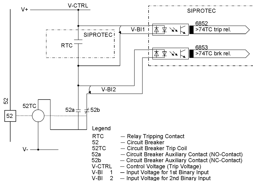
Figure 2-76 Principle of the trip circuit supervision with two binary inputs
