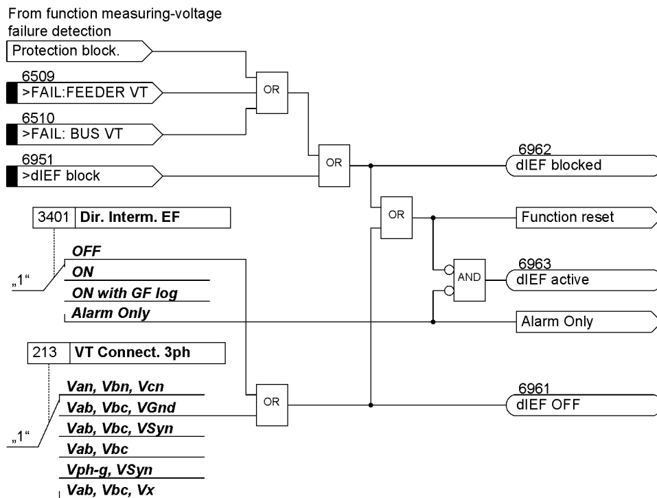
Figure 2-98 Activation of the directional intermittent ground fault protection
