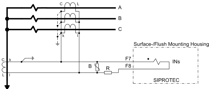
Figure A-20 High-impedance differential protection for a grounded transformer winding (the illustration shows the partial connection for high-impedance differential protection)
