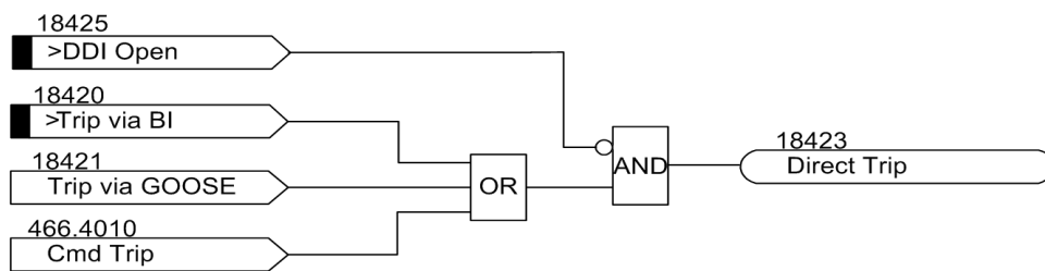
Figure 2-7 Logic diagram of PI Direct Trip
