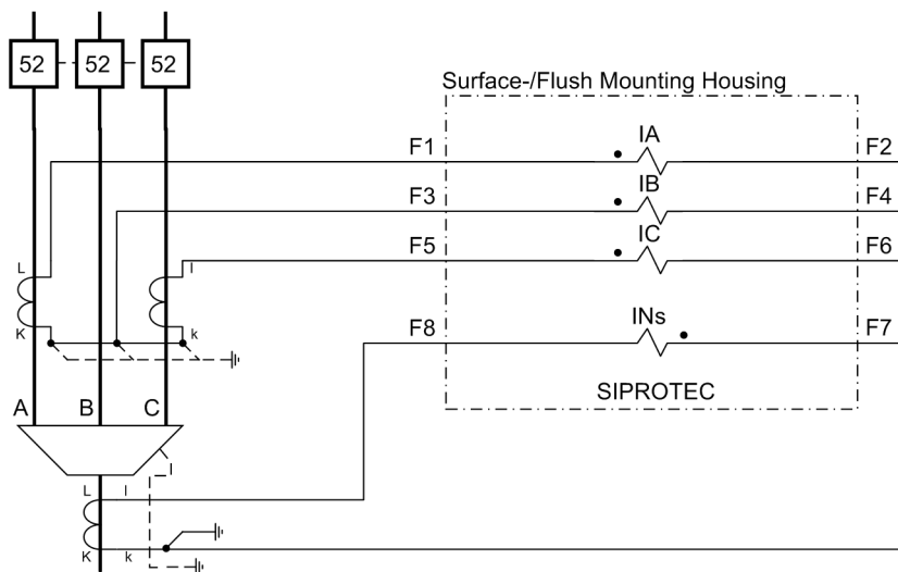
Figure A-10 Current transformer connections to two current transformers - additional cable-type current transformer for sensitive ground fault detection - only for isolated or resonant-grounded networks
