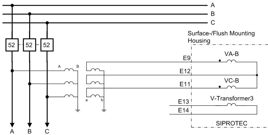
Figure A-26 Example for connection type "VAB, VBC"
