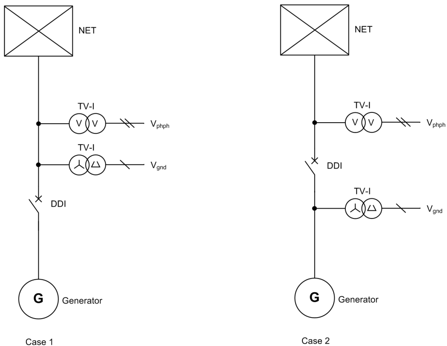
Figure 2-51 Application guide of VT installation position: Case 1 and Case 2
