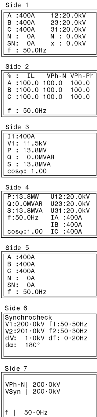
Figure A-31 Default display of the 7SJ80 for models with V without extended measured values
