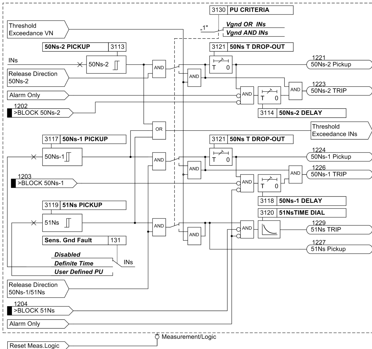
Figure 2-86 Logic diagram of the I_{Ns} elements during \cos \varphi / \sin \varphi measurement
