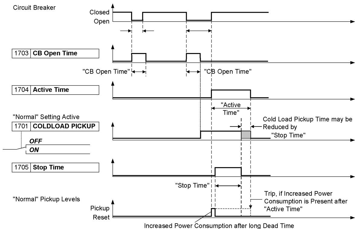
Figure 2-36 Timing charts of the dynamic cold load pickup function
