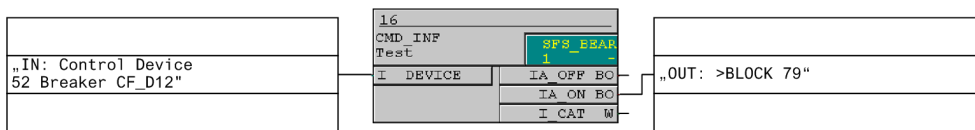
Figure 2-105 Blocking of the automatic reclose function using the internal control function
