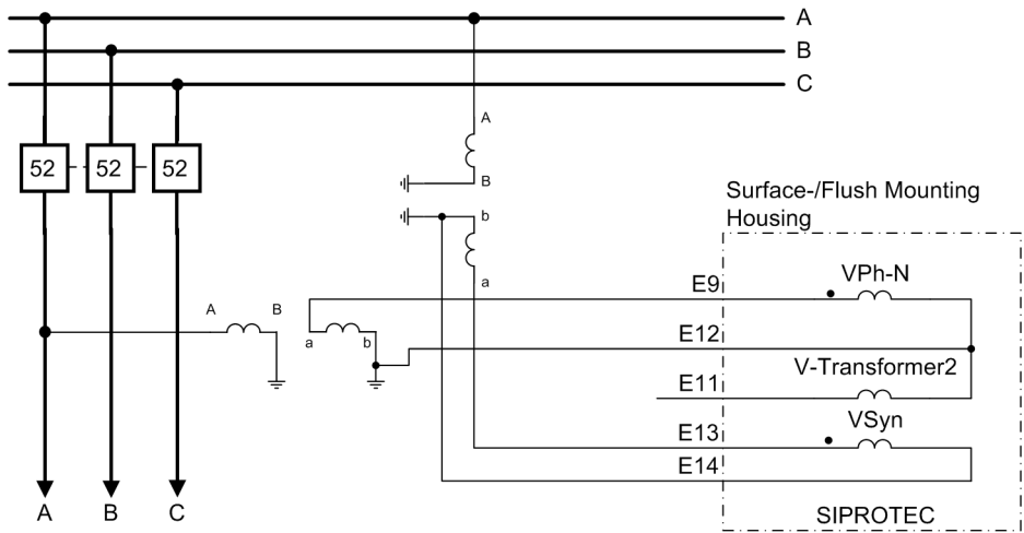
Figure A-24 Example for connection type "Vph-n, Vsyn"
