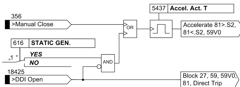
Figure 2-64 Logic diagram of accelerating feature
