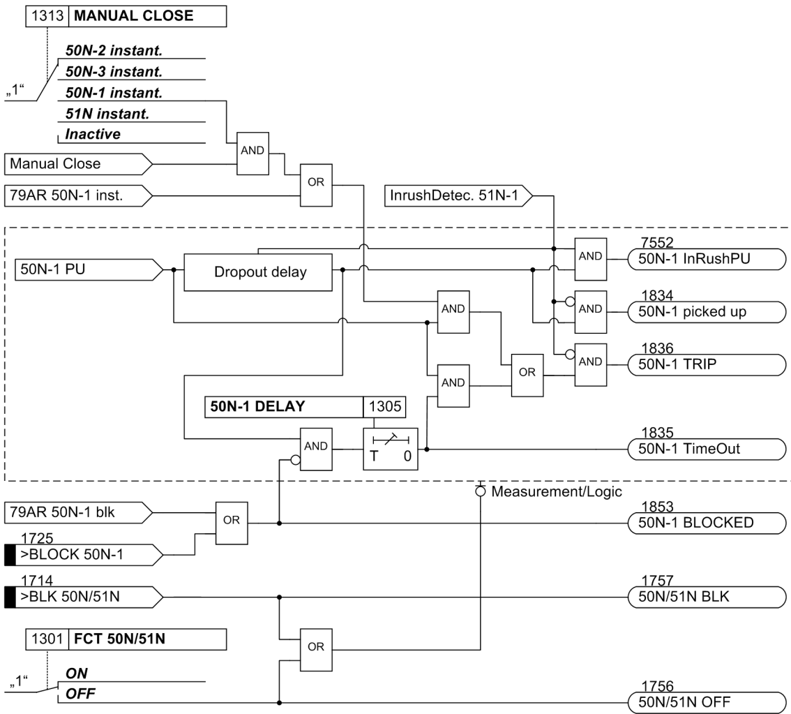
Figure 2-12 Logic diagram for the 50N-1 overcurrent current element
