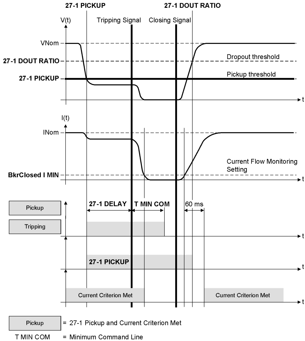
Figure 2-48 Typical fault profile for load side connection of the voltage transformers (with current supervision)
