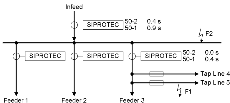
Figure 2-103 Zone sequencing with a fault occurring at Tap Line 5 and at the busbar
