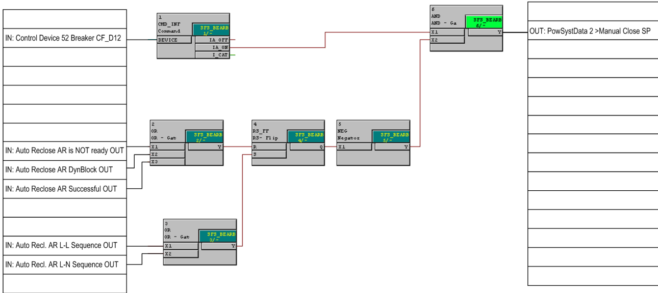
Figure 2-104 CFC logic for Manual Close with automatic reclosing via control
