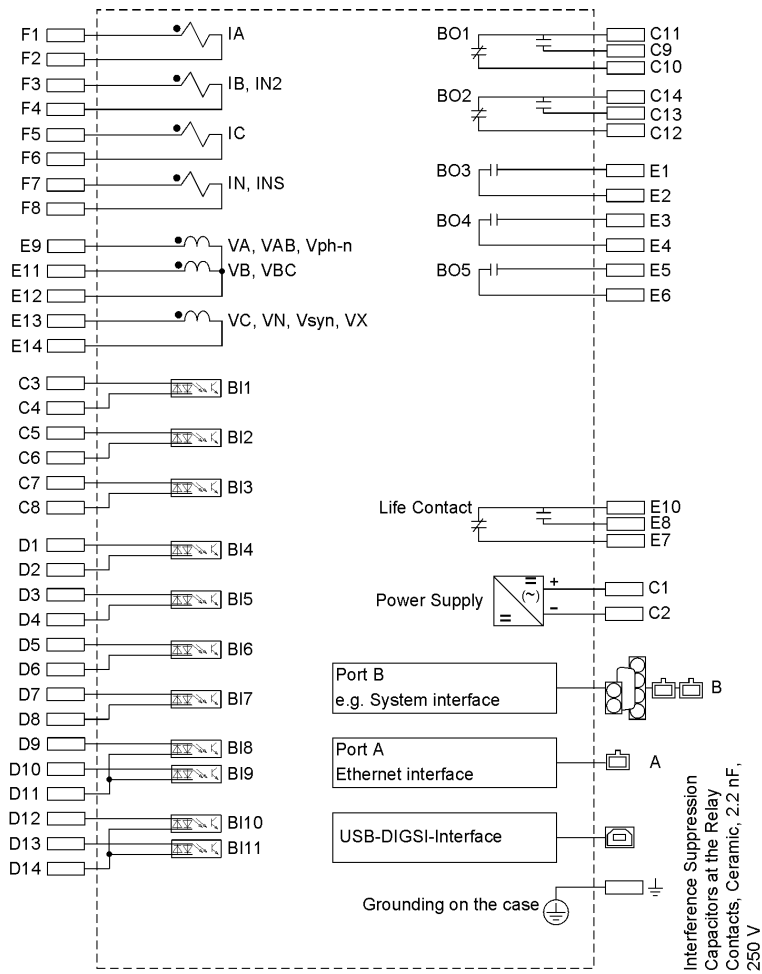
Figure A-6 Connection diagram 7SJ808*
