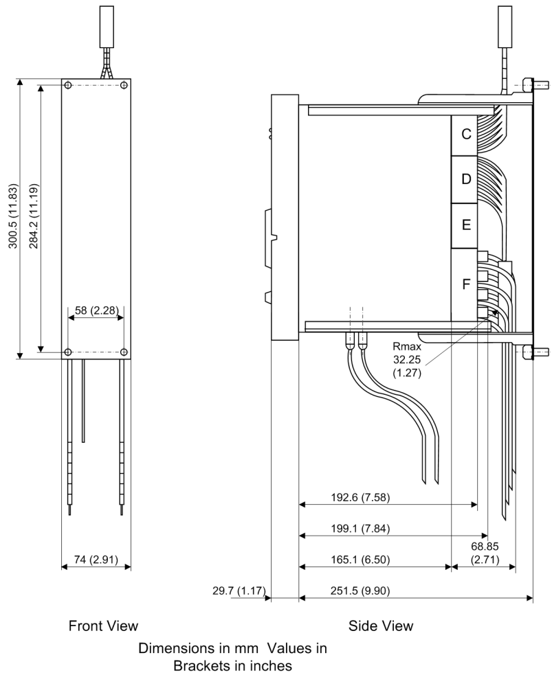
Figure 4-12 Dimensional drawing of a 7SJ80 for panel surface mounting (housing size 1/6)
