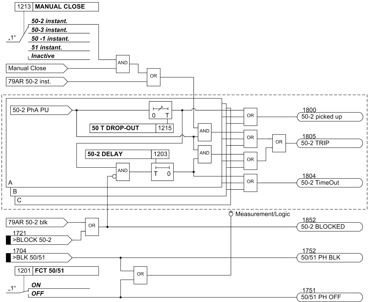
Figure 2-8 Logic diagram for 50-2 high-set element for phases
