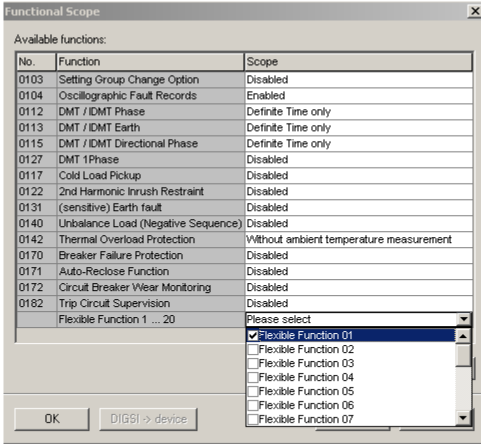
Figure 2-115 Configuration of a flexible protection function
