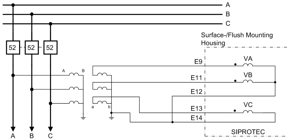
Figure A-21 Example for the connection type "VAN, VBN, VCN" with voltage connection on the feeder side
