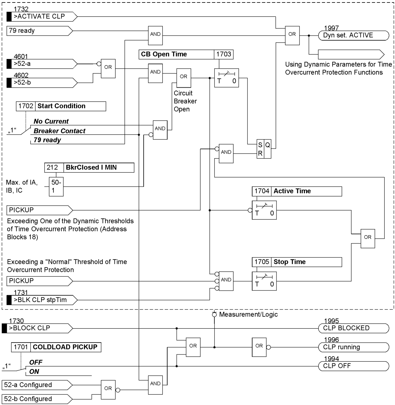
Figure 2-37 Logic diagram of the dynamic cold load pickup function (50c, 50Nc, 51c, 51Nc, 67c, 67Nc)
