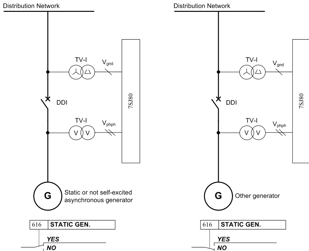
Figure 2-6 Static Generator
