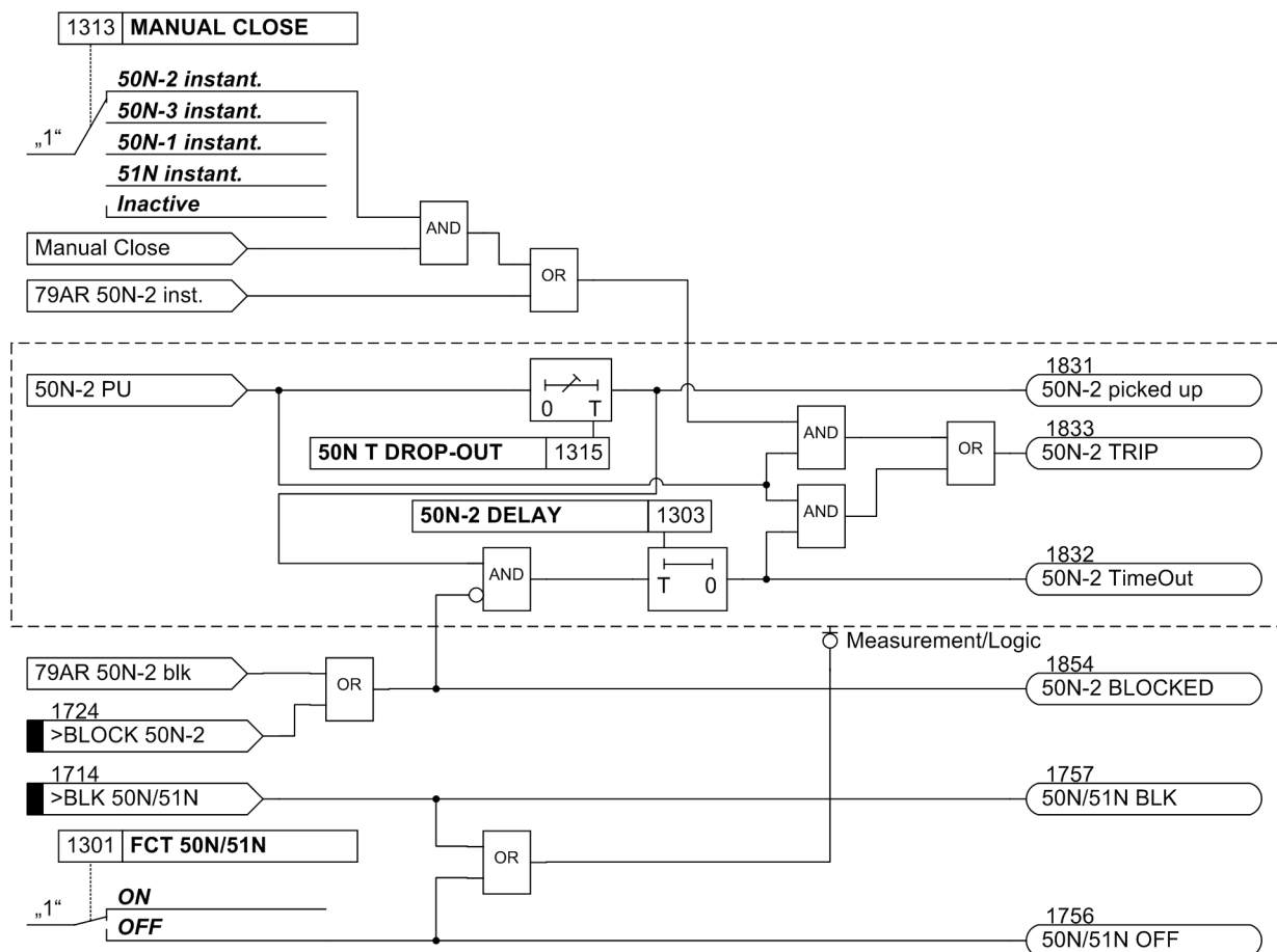
Figure 2-9 Logic diagram for 50N-2 high-set element
