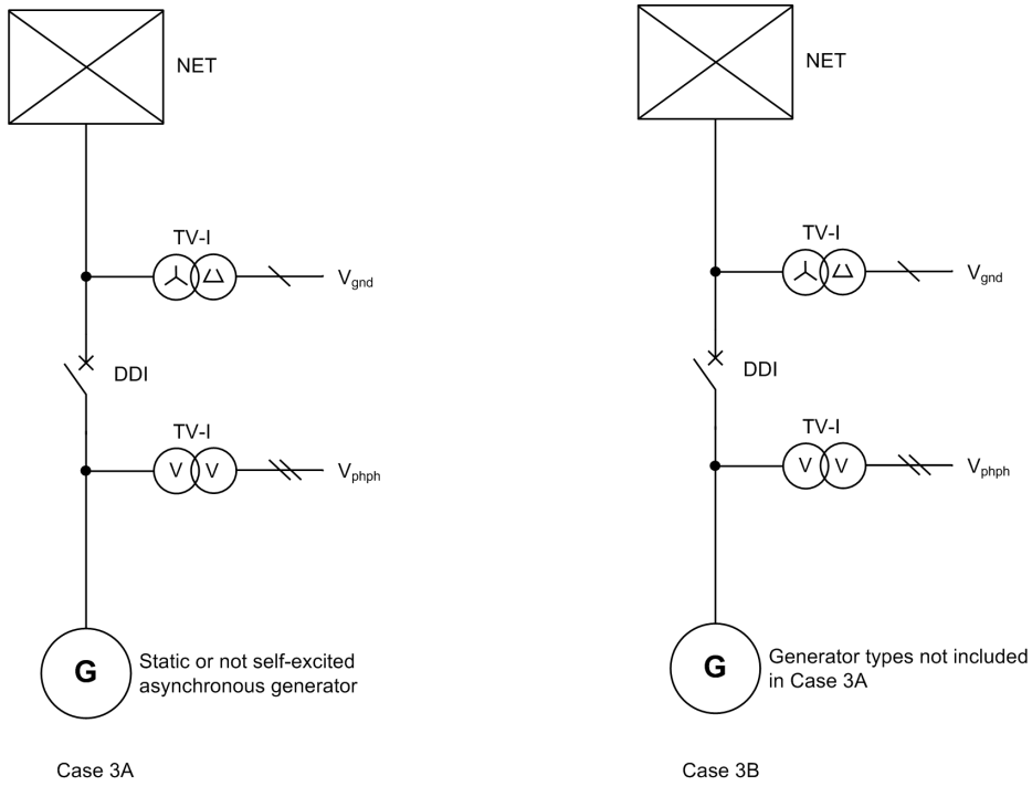
Figure 2-52 Application guide of VT installation position: Case 3
