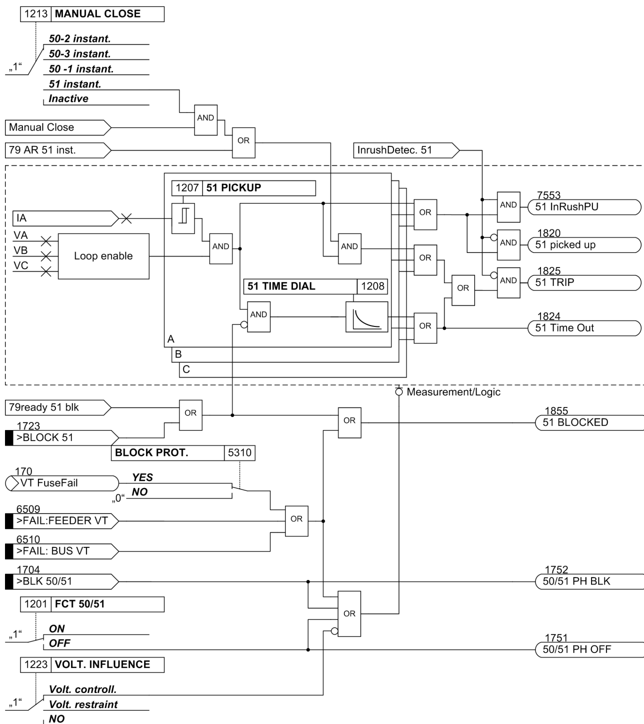
Figure 2-17 Logic diagram of the voltage-controlled inverse time overcurrent protection
