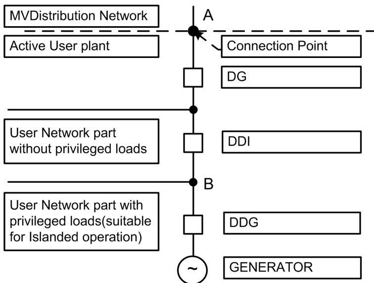
Figure 2-50 Primary main wiring of application
