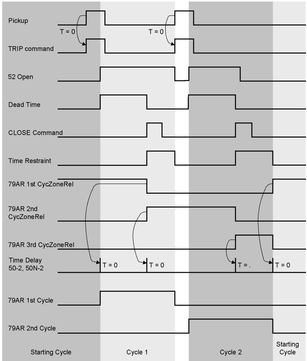
Figure 2-102 Control of protection elements for two-fold, successful automatic reclosure
