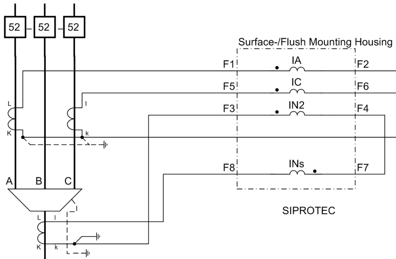
Figure A-18 Current transformer connections to two phase-current transformers and a ground-current transformer; the ground current is taken via the highly sensitive and sensitive ground input.
