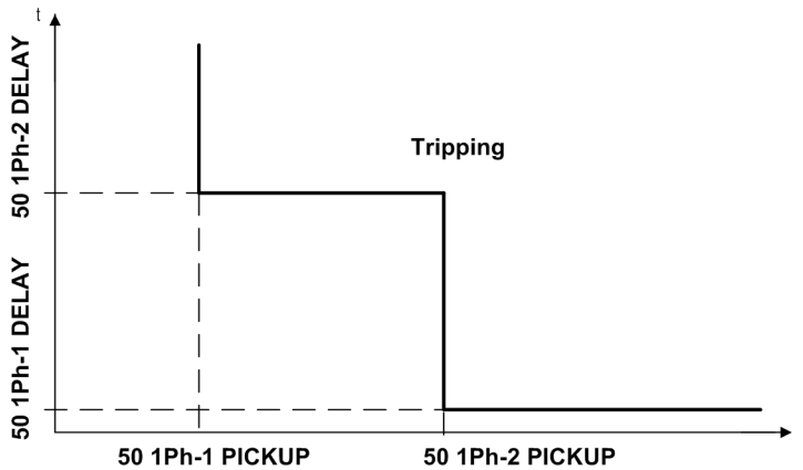
Figure 2-38 Two-stage characteristic of the single-phase time-overcurrent protection
