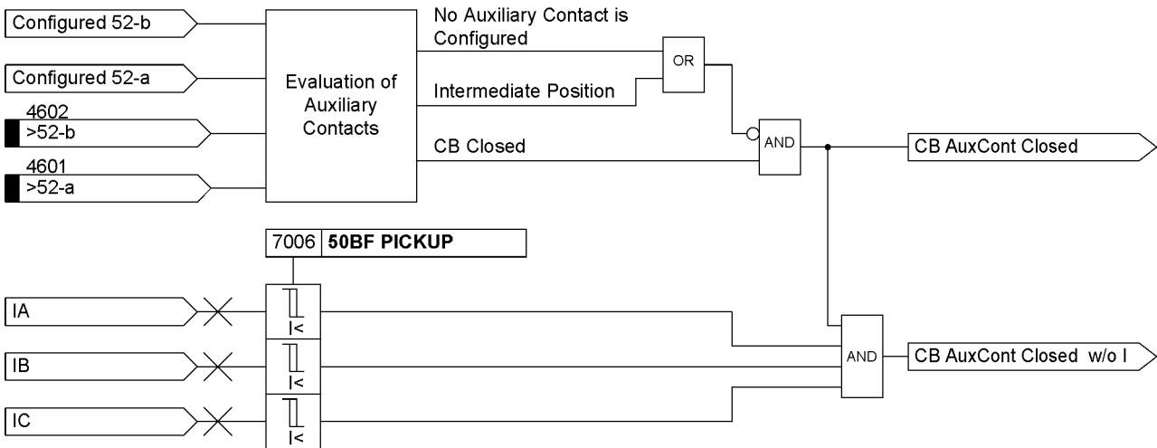
Figure 2-108 Logic diagram for breaker failure protection, monitoring of the circuit-breaker auxiliary contacts
