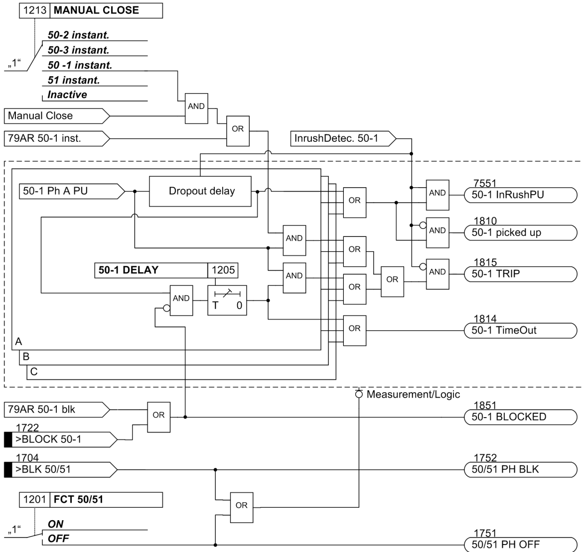
Figure 2-10 Logic diagram for the 50-1 overcurrent element for phases
