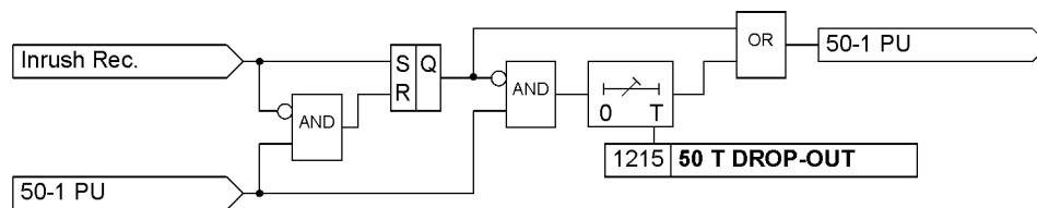
Figure 2-11 Logic diagram of the dropout delay for 50-1
