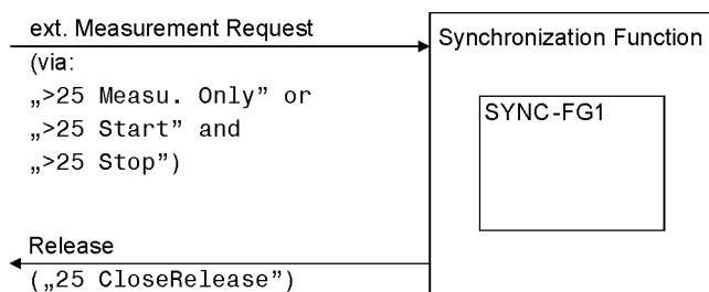
Figure 2-125 Interaction of synchrocheck function and external control
