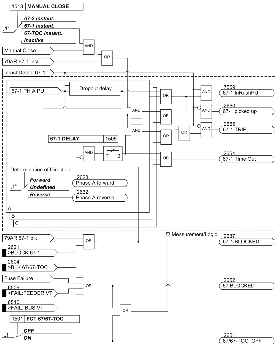
Figure 2-25 Logic diagram for the directional relay element 67-1 for phases
