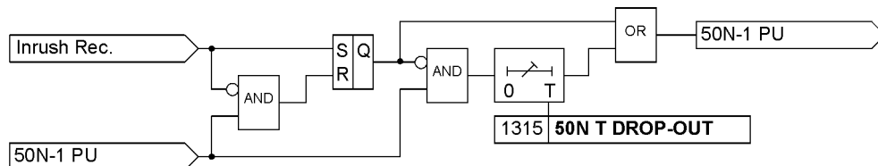
Figure 2-13 Logic of the dropout delay for 50N-1
