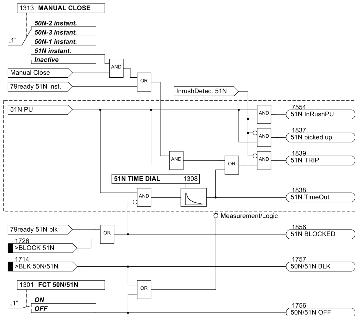
Figure 2-15 Logic diagram of the inverse-time overcurrent protection element for Ground
