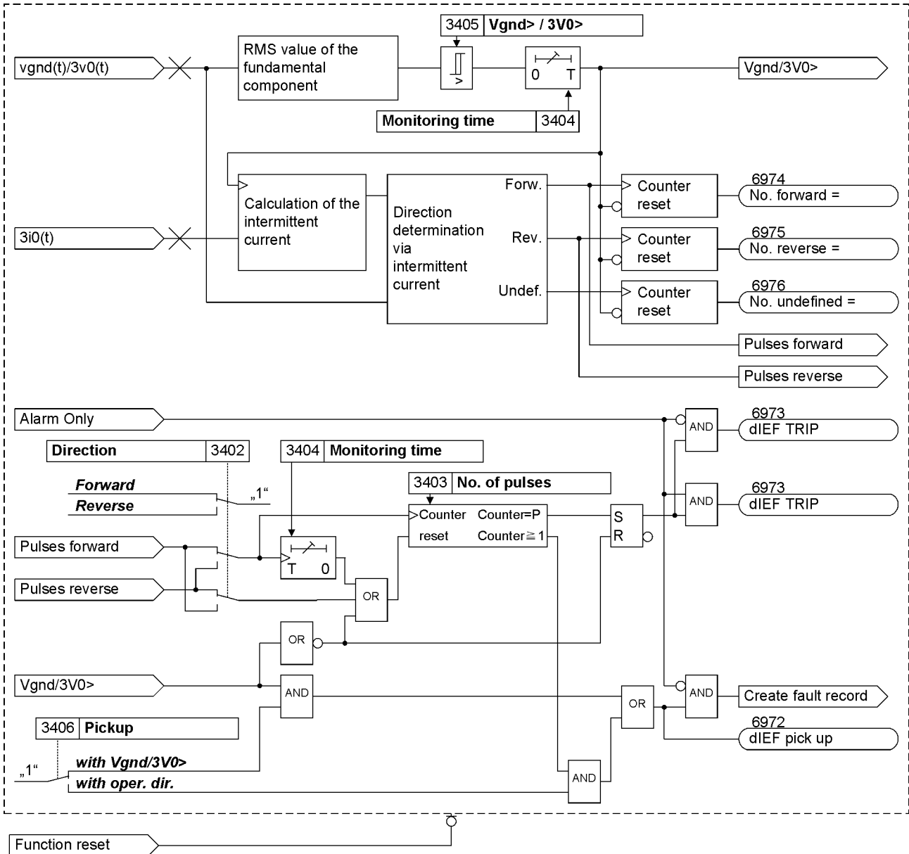
Figure 2-99 Logic diagram of the directional intermittent ground fault protection
