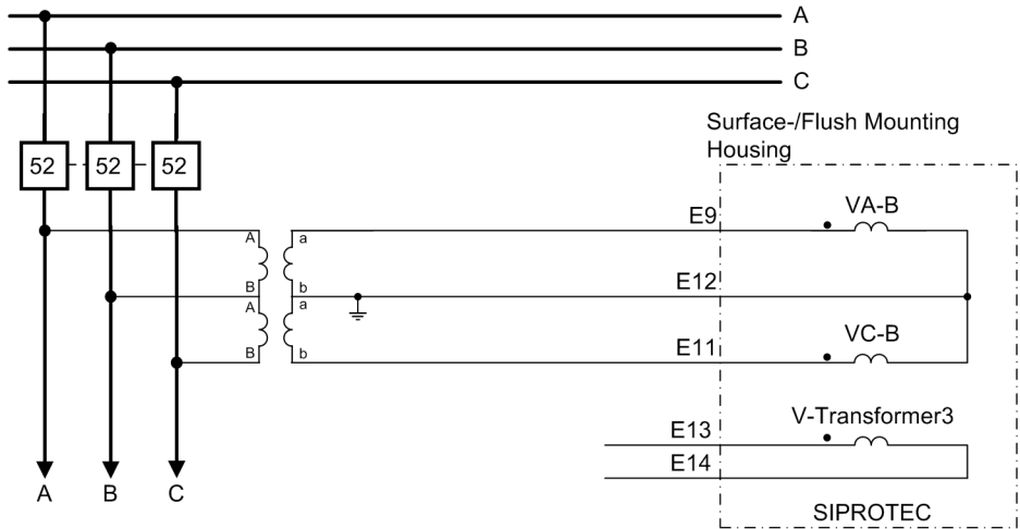
Figure A-27 Example for connection type "VAB, VBC" with phase voltage connection as open-delta connection
