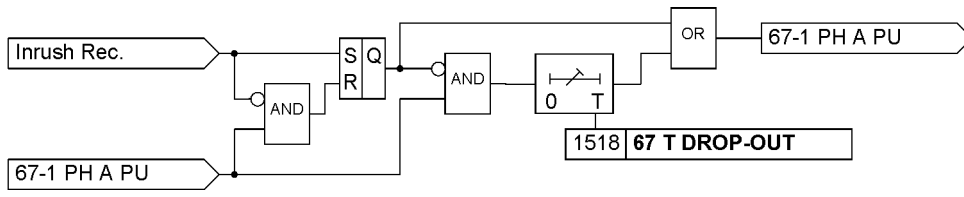
Figure 2-26 Logic of the dropout delay for 67-1
