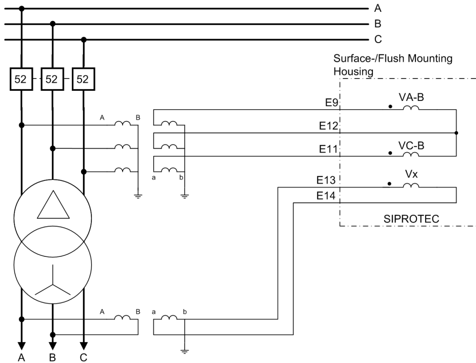
Figure A-25 Example for connection type "VAB, VBC, Vx"
