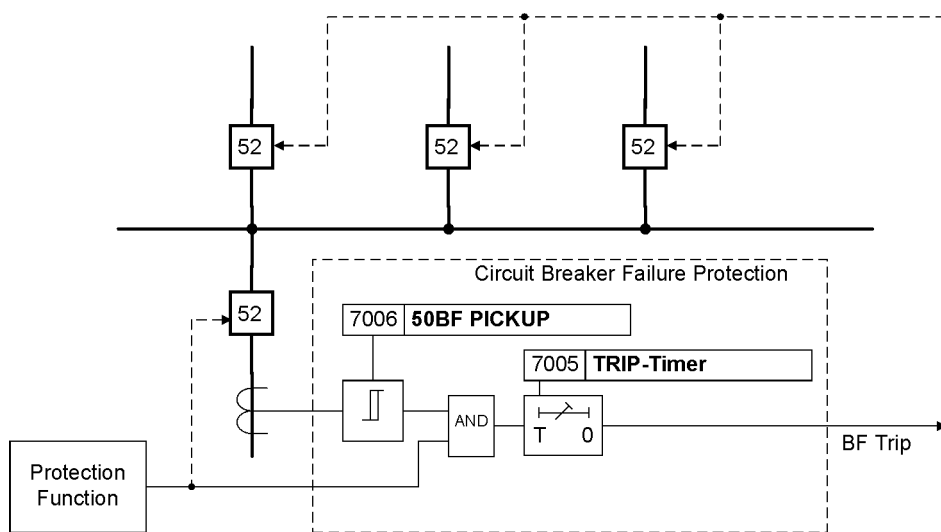
Figure 2-106 Function principle of the breaker failure protection
