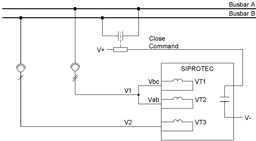
Figure 2-122 Cross coupling
