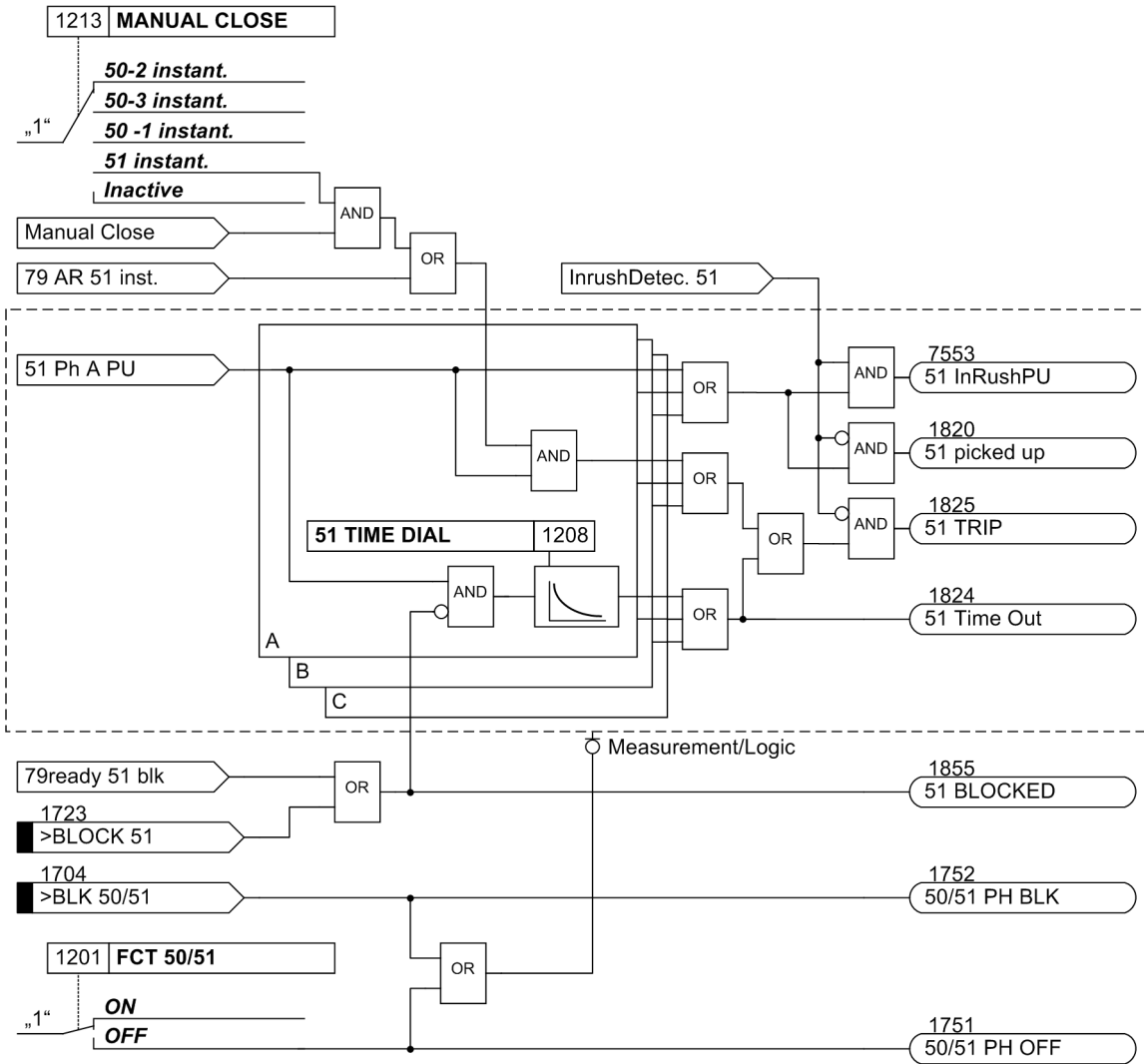
Figure 2-14 Logic diagram of the inverse-time overcurrent protection element for phases
