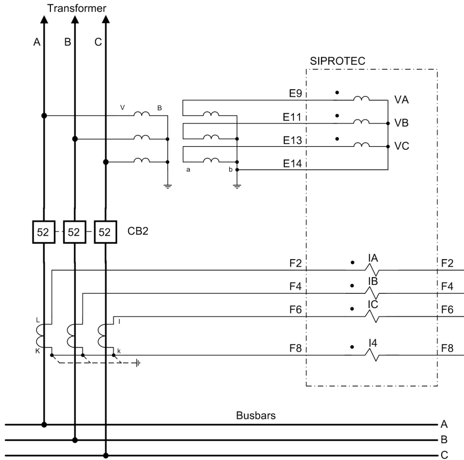
Figure 2-113 Wiring diagram for a 7SJ80 as reverse power protection
