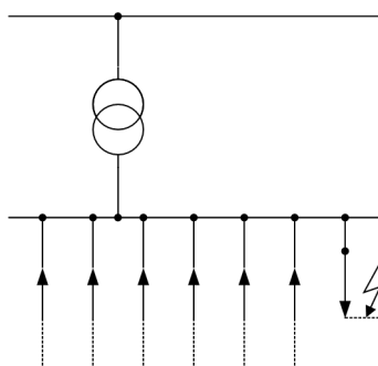
Figure 2-92 Location of ground faults in a radial network
