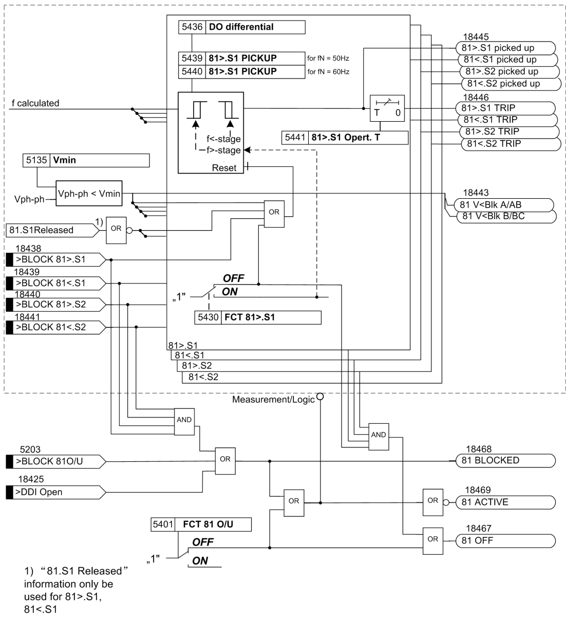
Figure 2-65 Logic diagram of the frequency protection
