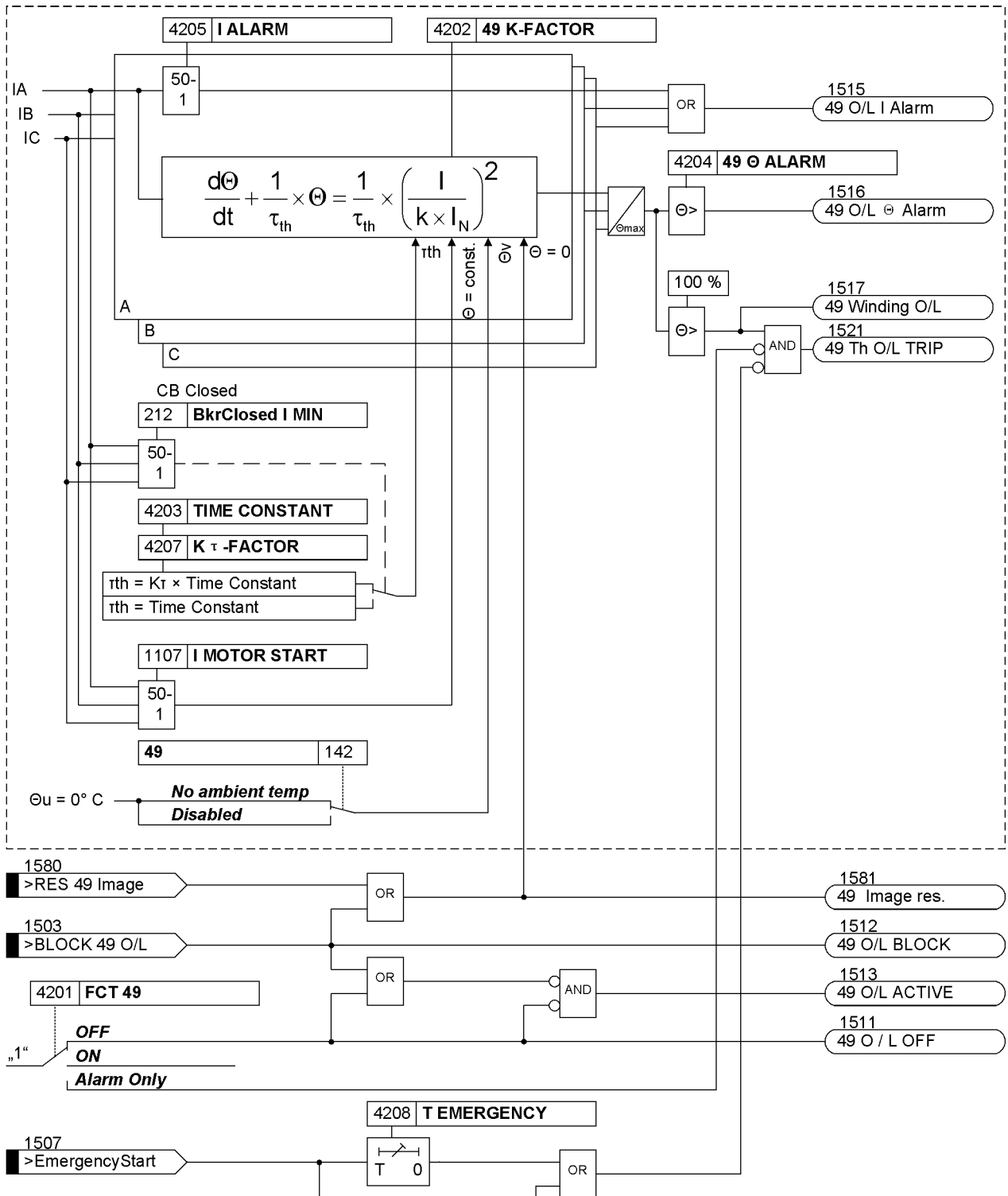
Figure 2-68 Logic diagram of the overload protection
