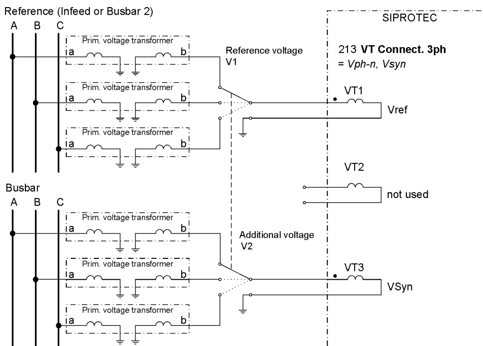
Figure 2-128 Phase-to-ground voltage connection
