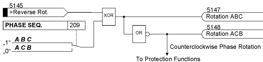
Figure 2-129 Message logic of the phase rotation reversal
