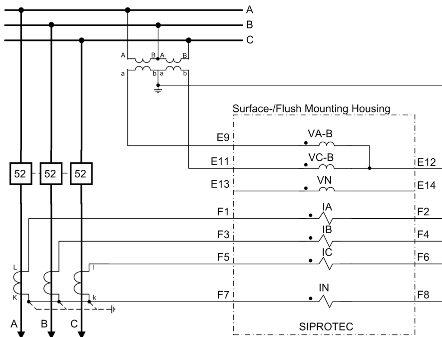
Figure A-16 Current transformer connections to three current transformers, two voltage transformers in open-delta connection, only for isolated or resonant-grounded networks; no directional ground protection since displacement voltage cannot be calculated
