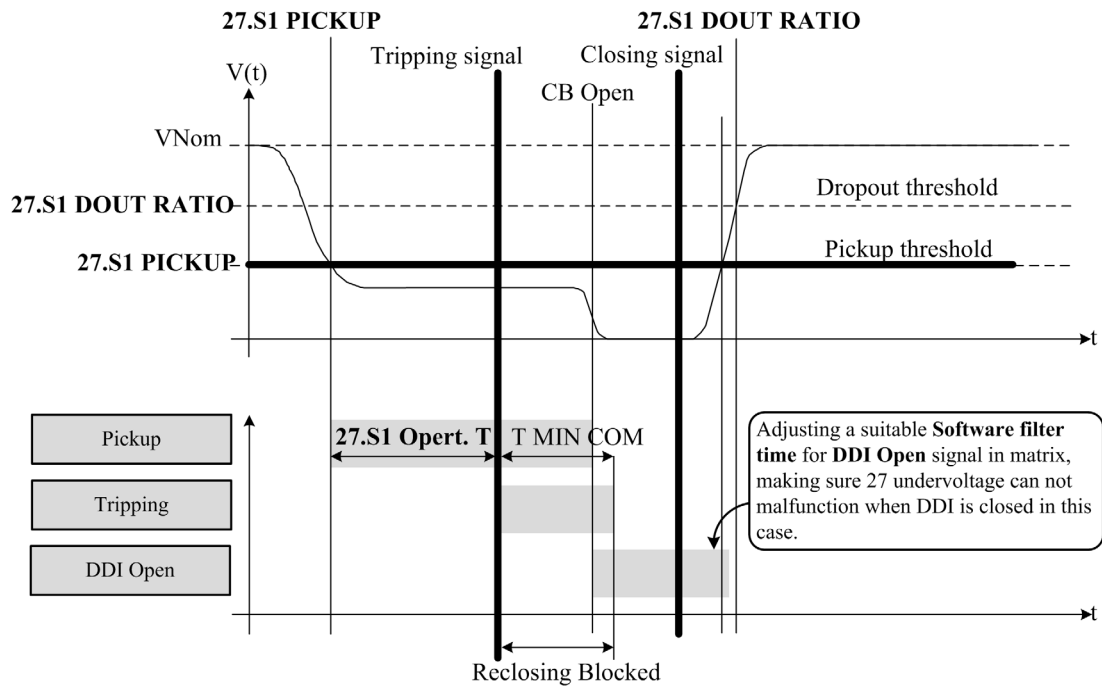
Figure 2-56 Typical fault(user side fault) profile for user side connection of the voltage transformers
