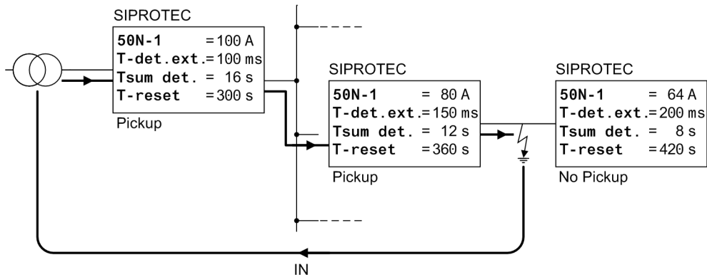
Figure 2-97 Example of selectivity criteria of the intermittent ground fault protection
