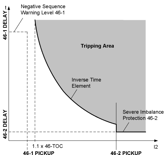
Figure 2-60 Inverse time characteristic for negative sequence protection
