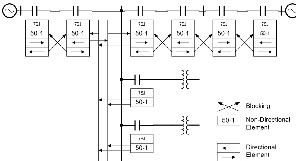
Figure 2-33 Reverse interlocking using directional elements
