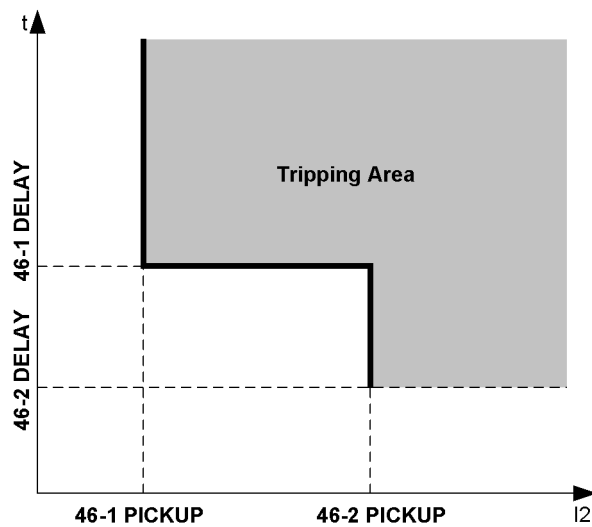
Figure 2-59 Definite time characteristic for negative sequence protection
