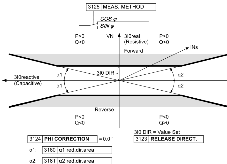
Figure 2-82 Directional characteristic for \cos\varphi -measurement
