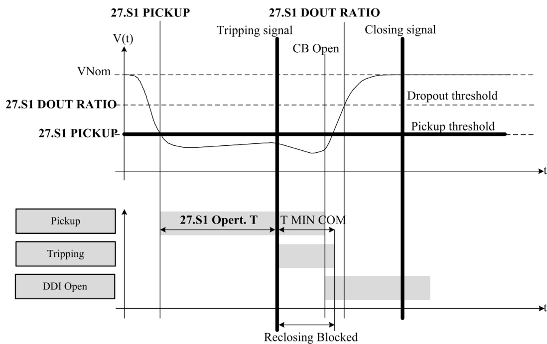
Figure 2-57 Typical fault (source side fault) profile for user side connection of the voltage transformers
