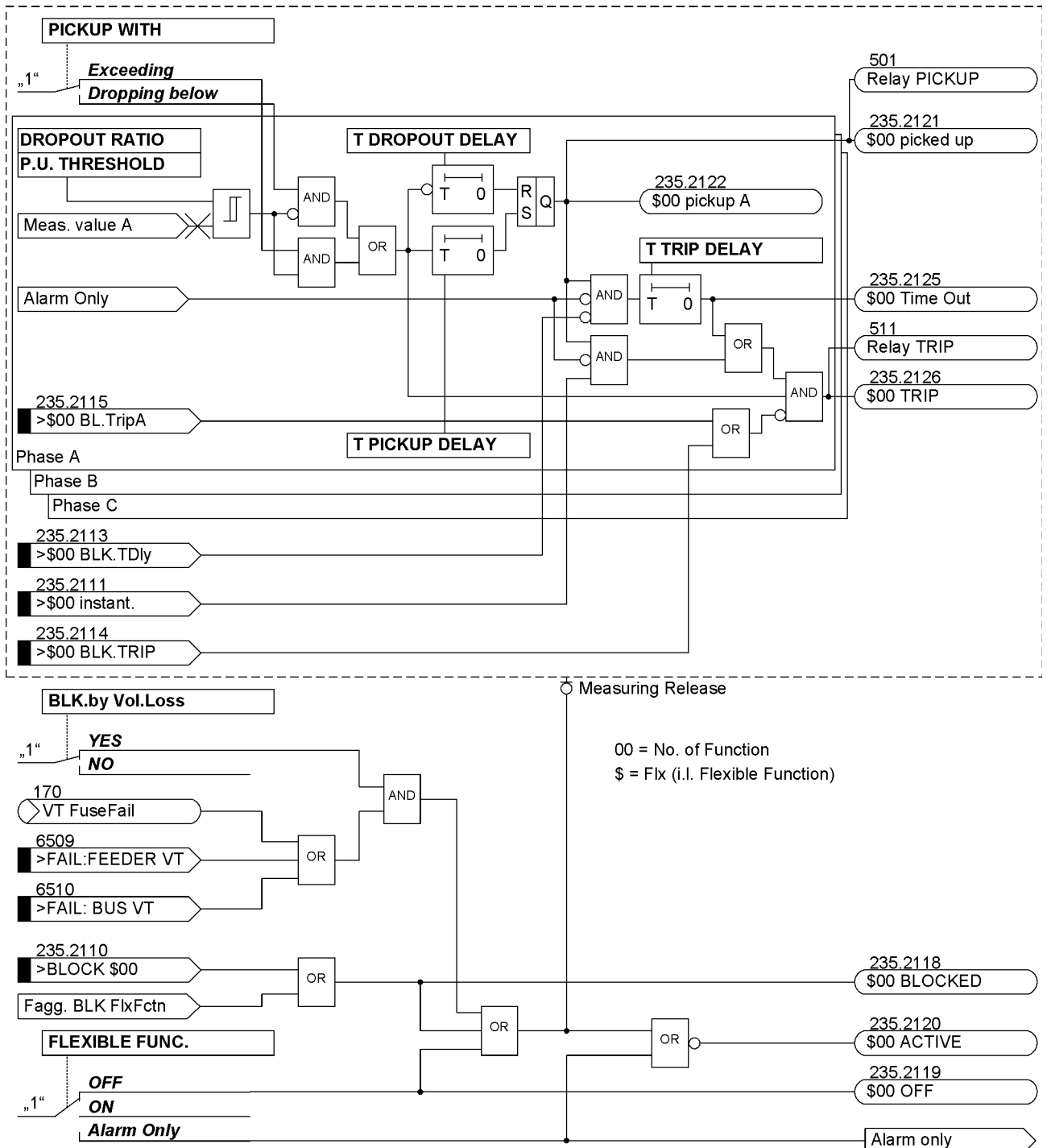
Figure 2-111 Logic diagram of the flexible protection functions
