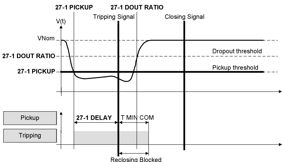
Figure 2-47 Typical fault profile for source side connection of the voltage transformer (without current supervision)
