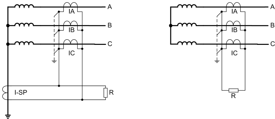
Figure 2-40 Ground fault protection according to the high-impedance principle
