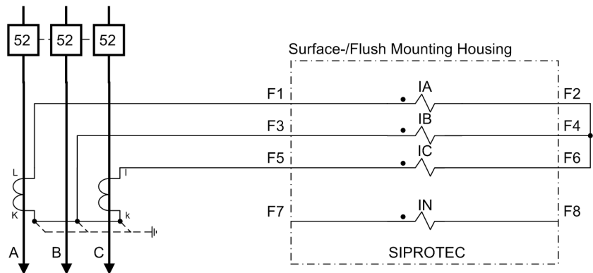
Figure A-8 Current transformer connections to two current transformers – only for isolated or resonant-grounded networks
