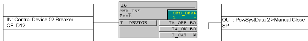
Figure 2-35 Example for the generation of a manual close signal using the internal control function
