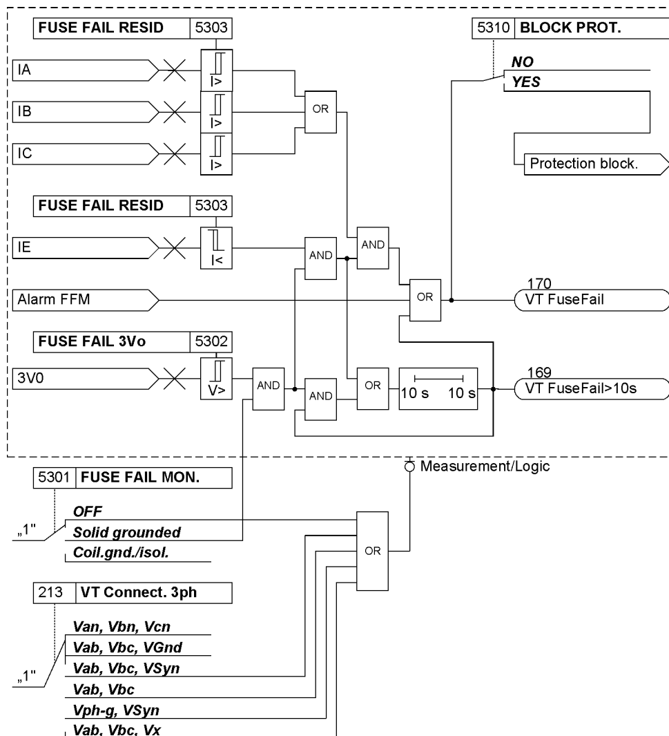
Figure 2-73 Logic diagram of the fuse failure monitor for grounded networks
