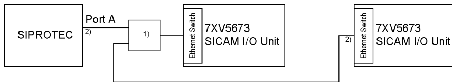
Figure A-30 Connection of 2 SICAM I/O units to port A via Y cable (up to 2 SICAM I/O units connectable)
