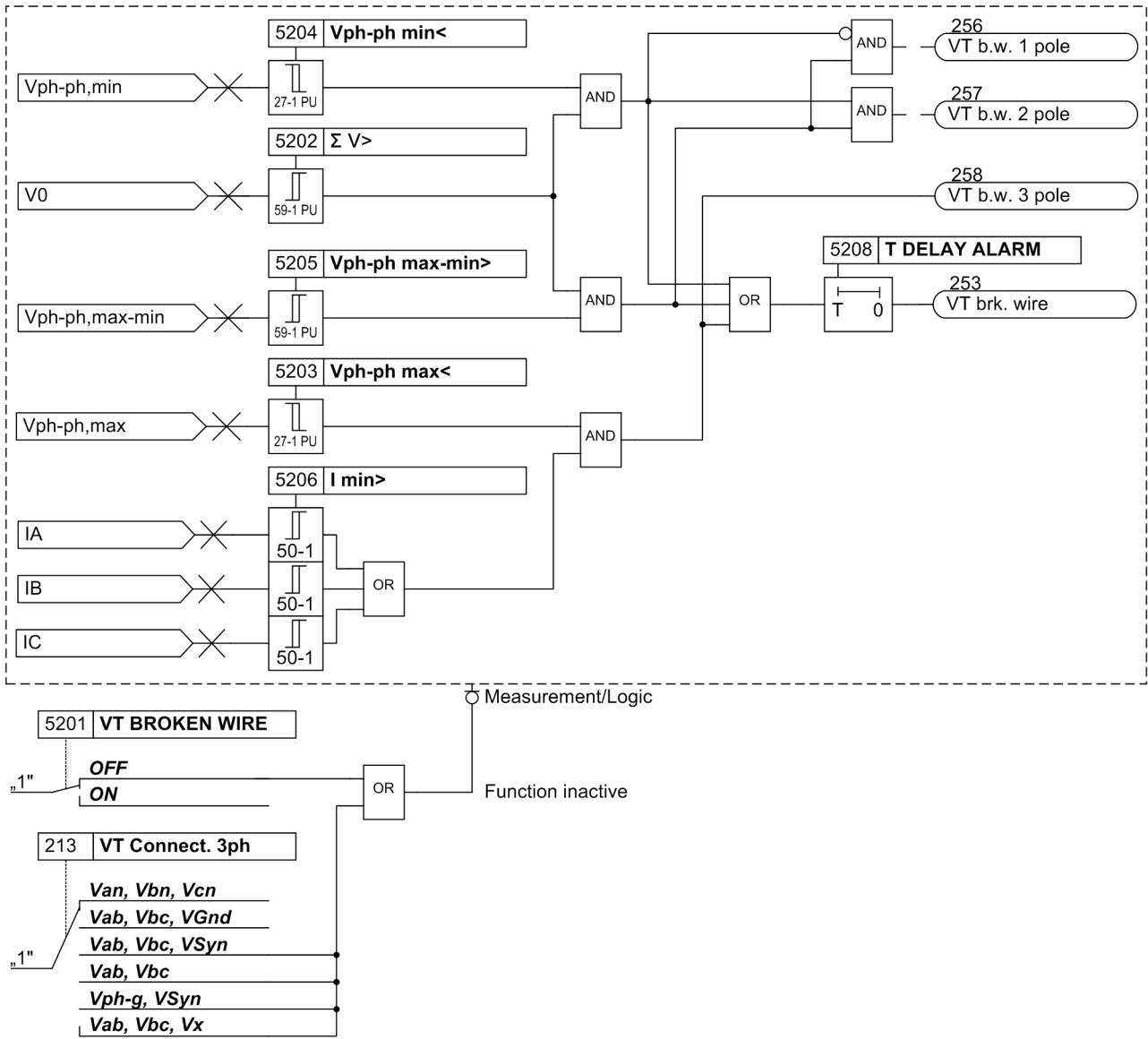
Figure 2-75 Logic diagram of the broken wire monitoring
