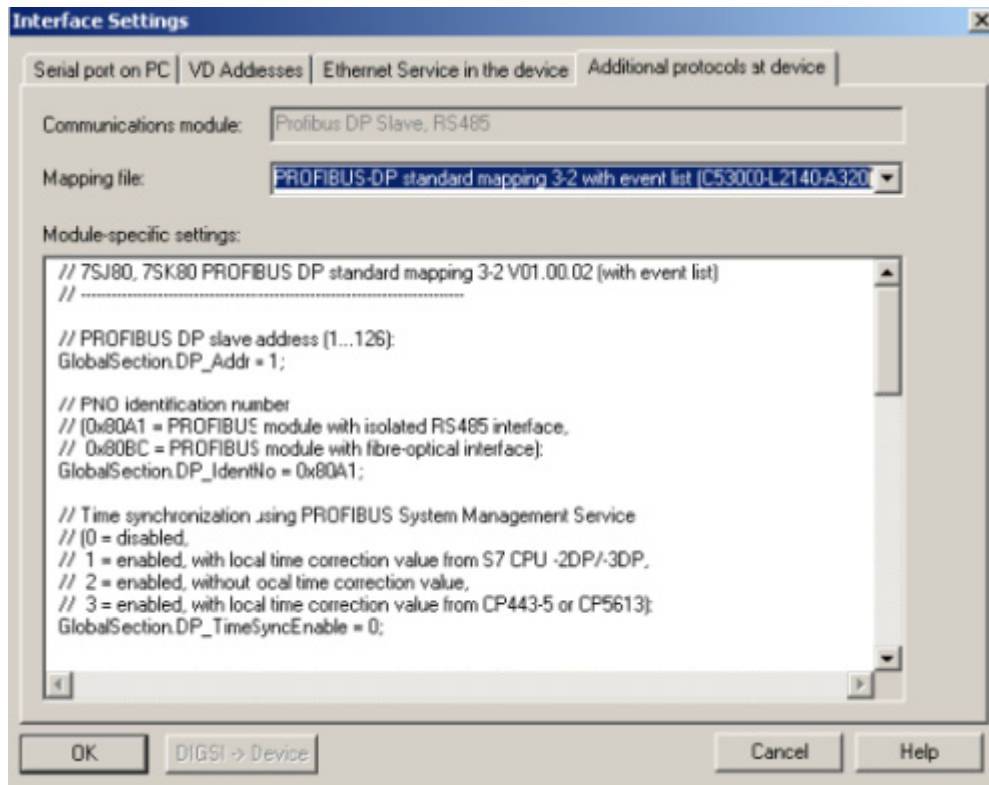
Figure 3-22 Module-specific settings
