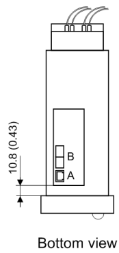
Figure 4-13 Bottom view of a 7SJ80 (housing size 1/6)
