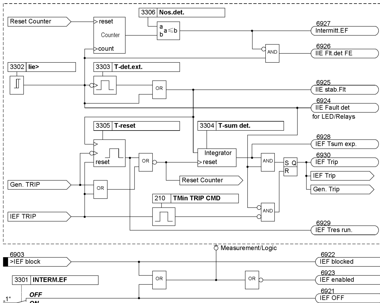
Figure 2-96 Logic diagram of the intermittent ground fault protection – principle
