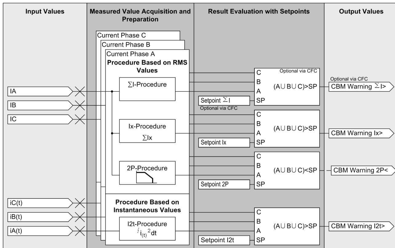
Figure 2-132 Diagram of CB maintenance procedures
