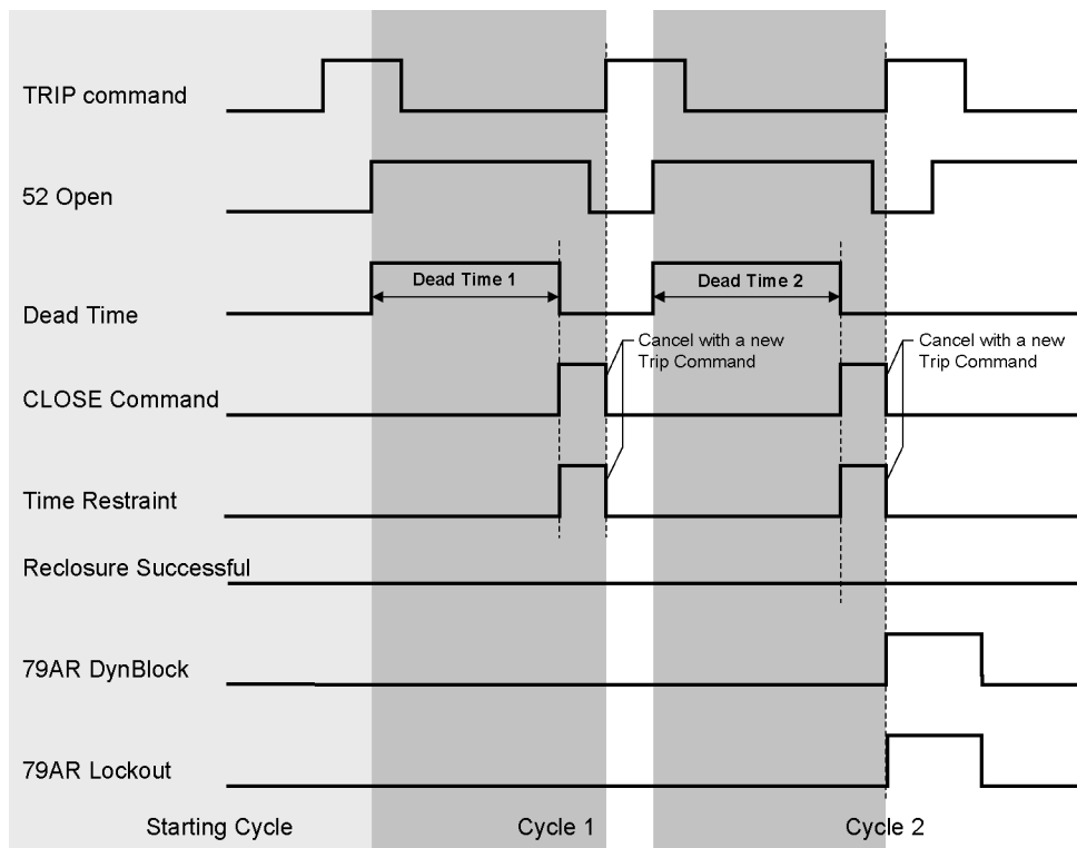
Figure 2-101 Timing diagram showing two unsuccessful reclosing shots
