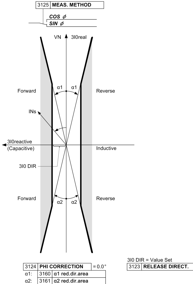
Figure 2-95 Directional characteristic for sin-φ-measurement
