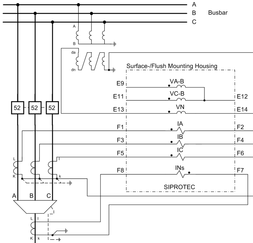
Figure A-17 Transformer connections to three current transformers, cable-type current transformer and broken delta winding, maximum precision for sensitive ground fault detection
