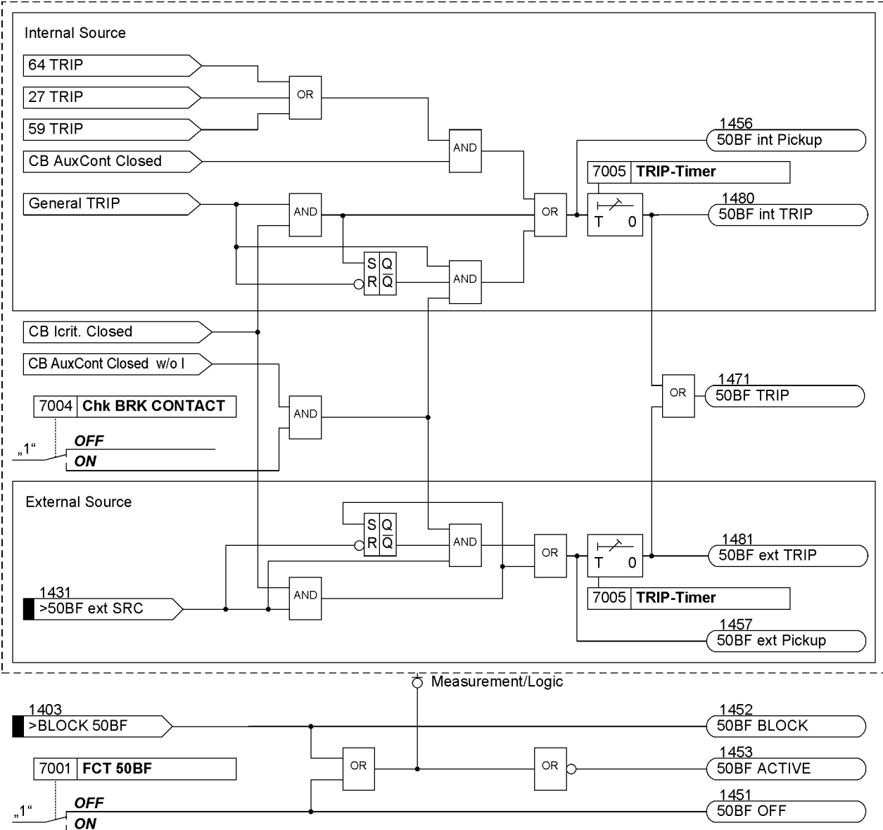
Figure 2-109 Logic diagram of the breaker failure protection
