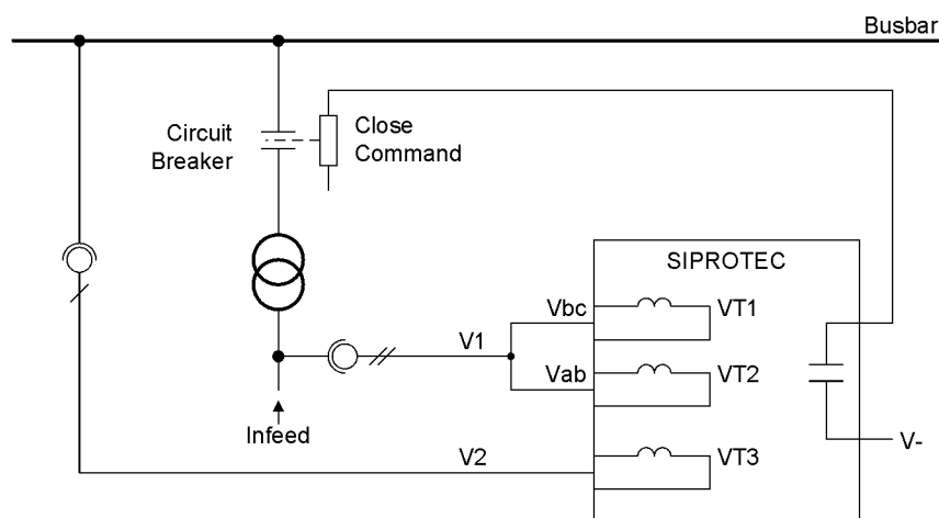
Figure 2-121 Infeed
