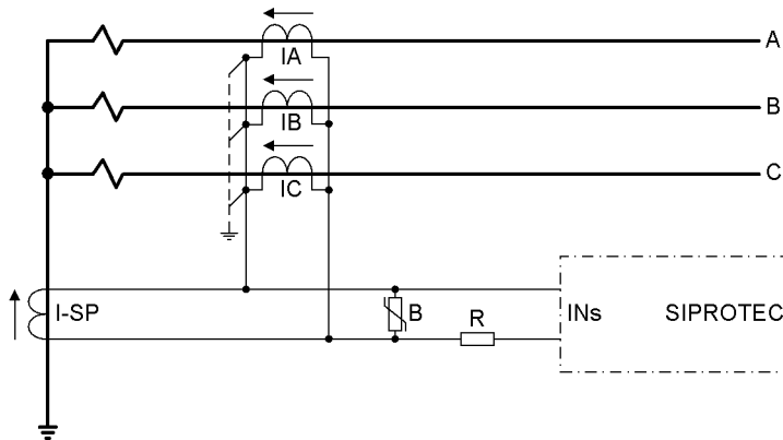
Figure 2-42 Connection scheme of the ground fault differential protection according to the high impedance principle
