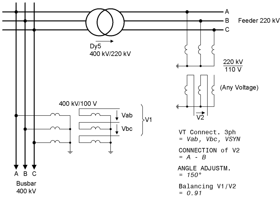
Figure 2-126 Busbar voltage measured across the transformer
