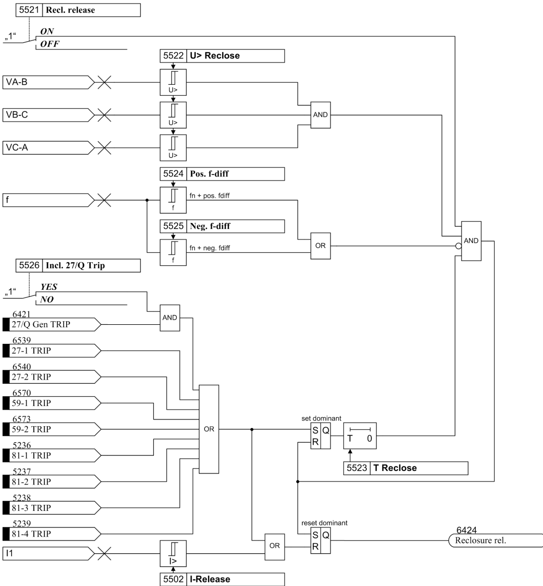
Figure 2-67 Logic diagram of QU protection restarting
