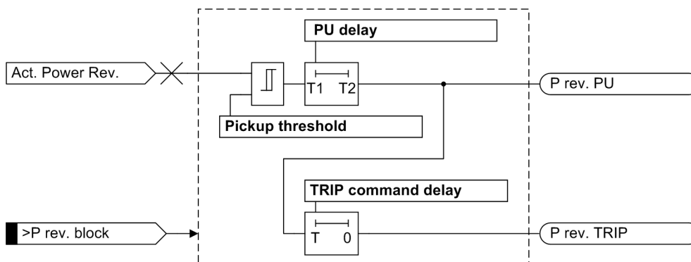
Figure 2-114 Logic diagram of the reverse power determination with flexible protection function
