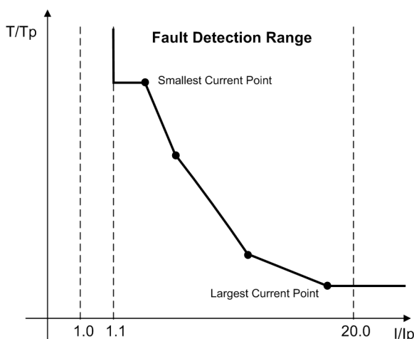
Figure 2-94 Use of a user-defined Curve
