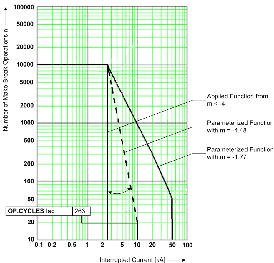
Figure 2-135 Value limitation of directional coefficient
