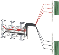
3KC9822-1
