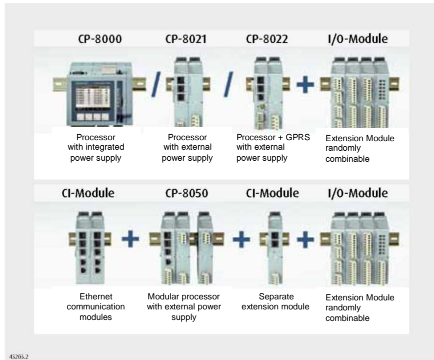
Fig. 2. The Sicam A8000 series is a module combination of processor, energy supply and expansion modules for inputs and outputs.
