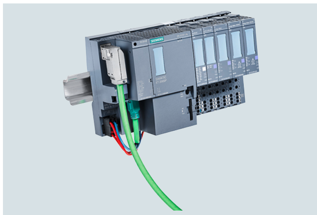
Mounting on the SIMATIC ET 200SP
