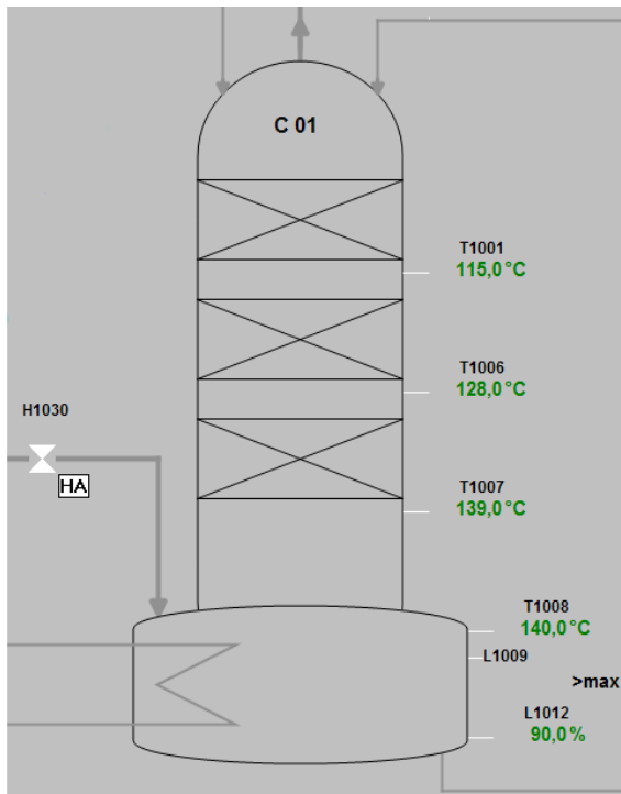
Fig. 4: Typical view of a distillation column
