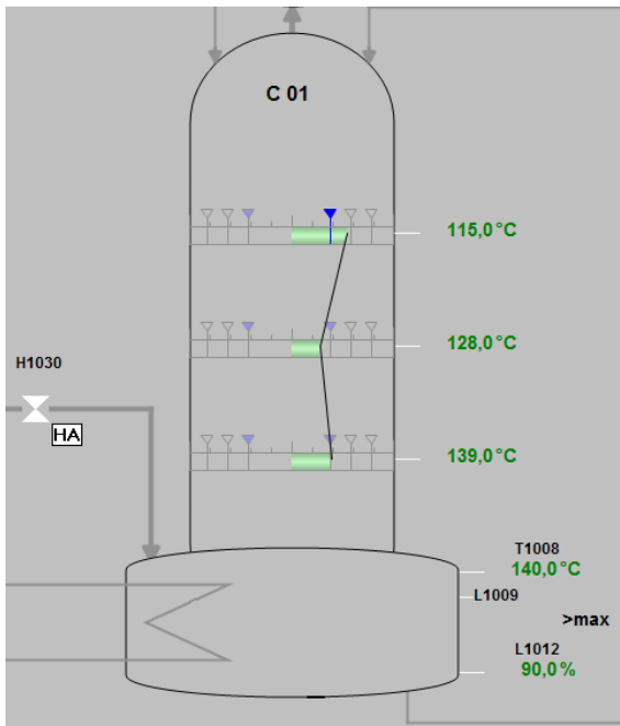
Fig. 5: View of a distillation column with vertical temperature curve
