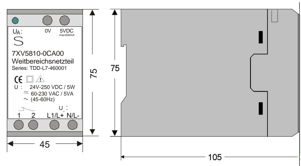
Abb. 4: Dimension Drawings
