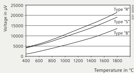
Characteristics for sensor types S, R and B
