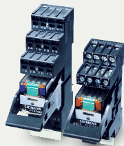
LZS:PT 2, 3 or 4 CO contacts AC-1: 12/10/6 A Width: 28 mm
