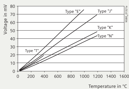
Characteristics for sensor types J, K, T, E and N
