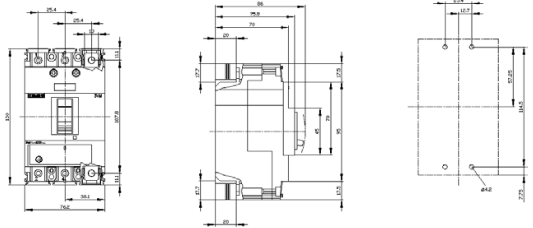
> 3VM10/11
