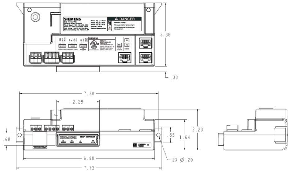
Controller Dimensions
