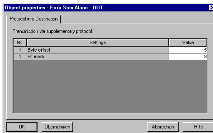
Figure 6-2 Definition of the position of an information in the PROFIBUS-DP message
