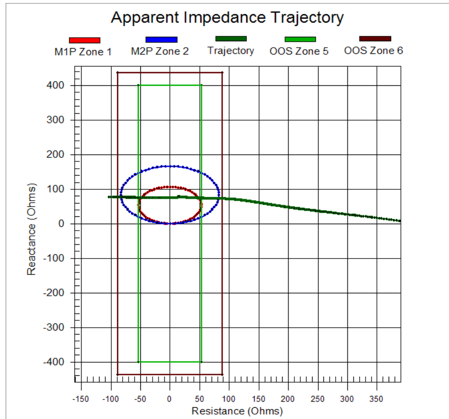
The apparent impedance trajectory enters the relay characteristic from the right. The out-of-step blinders measure the impedance traveling speed and declare a stable power swing condition. Therefore, the operations of Zone 1 and 2 distance protection have been blocked.
