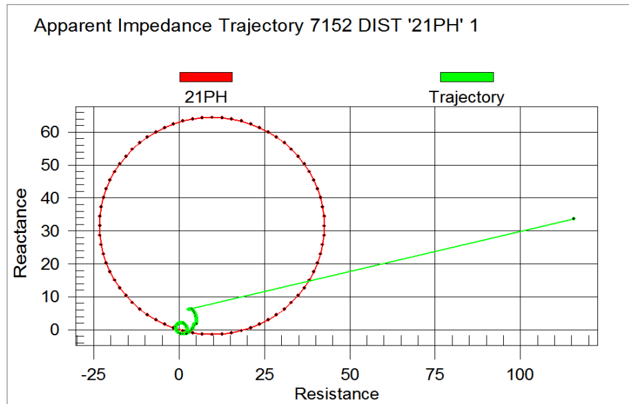
Above, trajectory of the apparent impedance measured by a distance relay. The apparent impedance enters the relay characteristic from the right. Below, a closer look at the trajectory.
