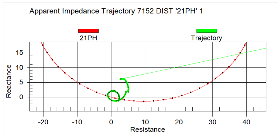
PSS®CAPE-TS Link's simulation platform allows study of the impact of protective relay switching on the overall dynamic behavior of the system.
