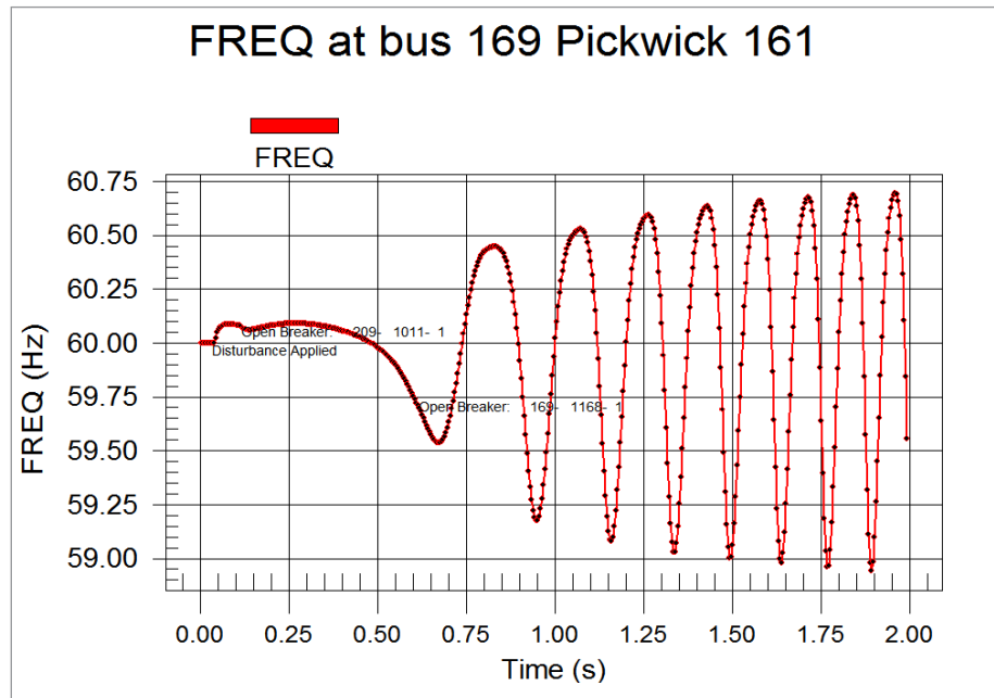
PSS®CAPE-TS Link output showing a plot of the frequency at a bus, including annotations.
