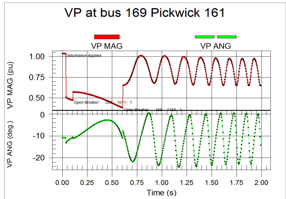
PSS®CAPE-TS Link output showing a plot of the voltage magnitude and angle at a bus, including annotations for when the disturbance was applied, and when breakers opened. This particular simulation results in instability after the fault is cleared, as evidenced by the oscillation in the magnitude of the voltage.
