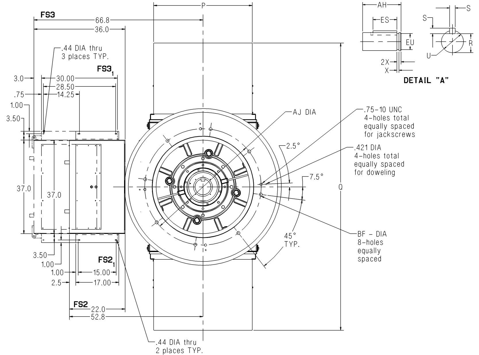
Standard Dimensions in Inches
