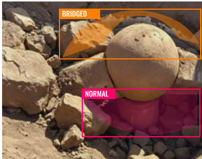
Crusher Bridging
