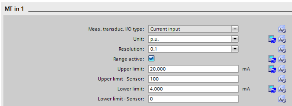
Fig.3: Configuration of input currents and measurement value range.
