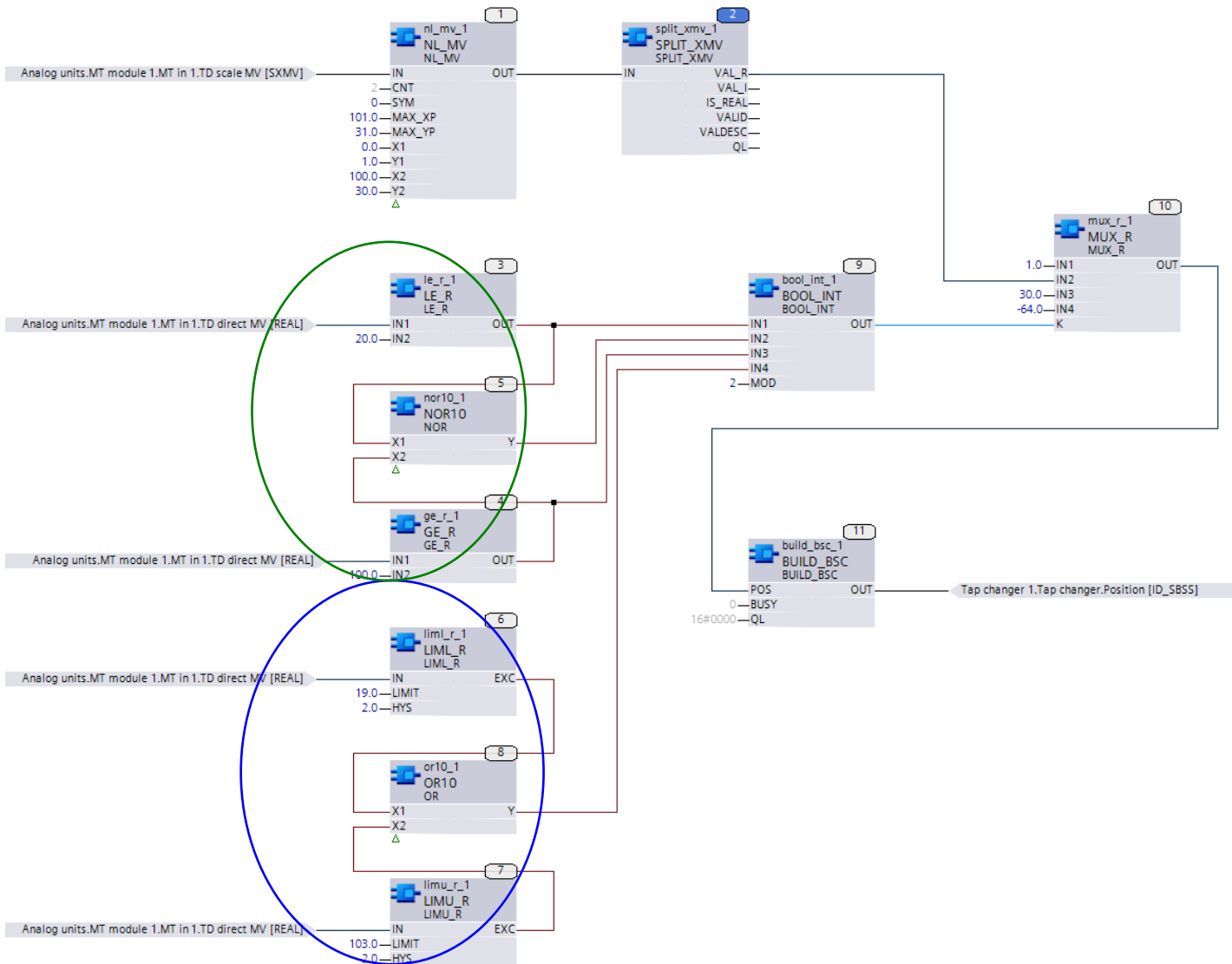
Fig.7: Complete CFC logic for the transformation including the handling of invalid input signals.
