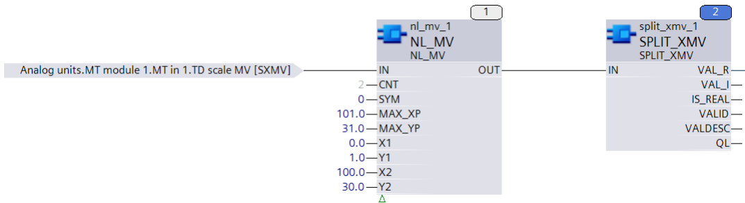
Fig.5.1: scaling the values for the correct tap positions.
