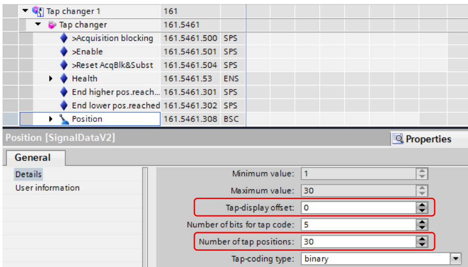
Fig.2: Setting the number of tap position and resulting minimum and maximum tap position
