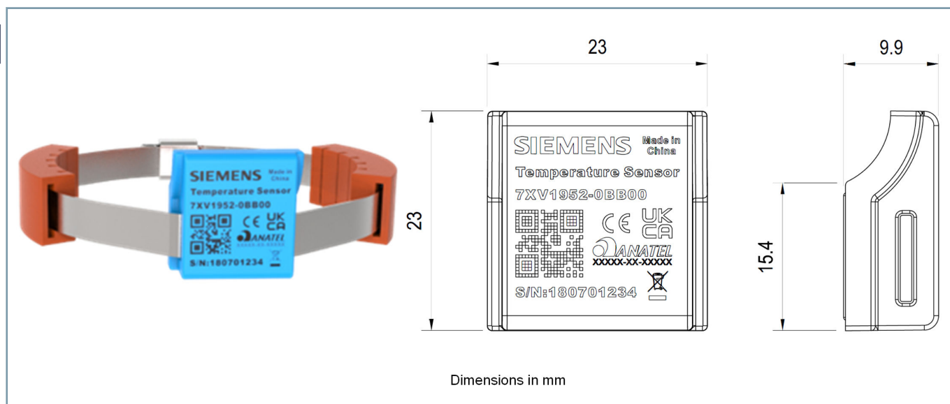
Figure 4.2/3 Wireless Sensor Dimensions
