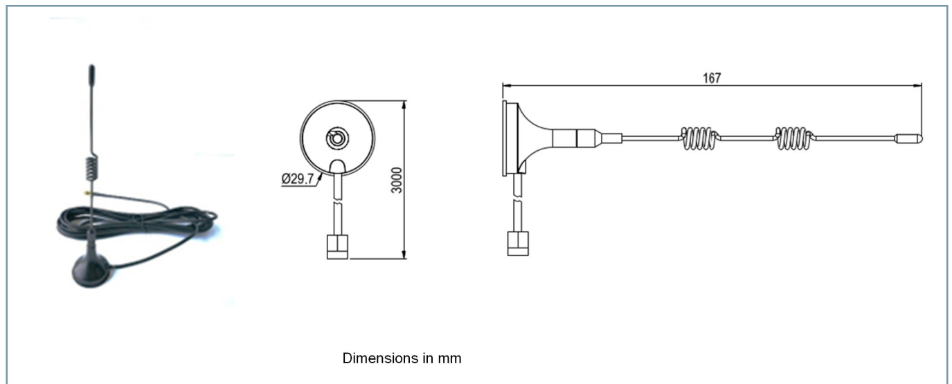
Figure 4.2/6 High-Gain Antenna
