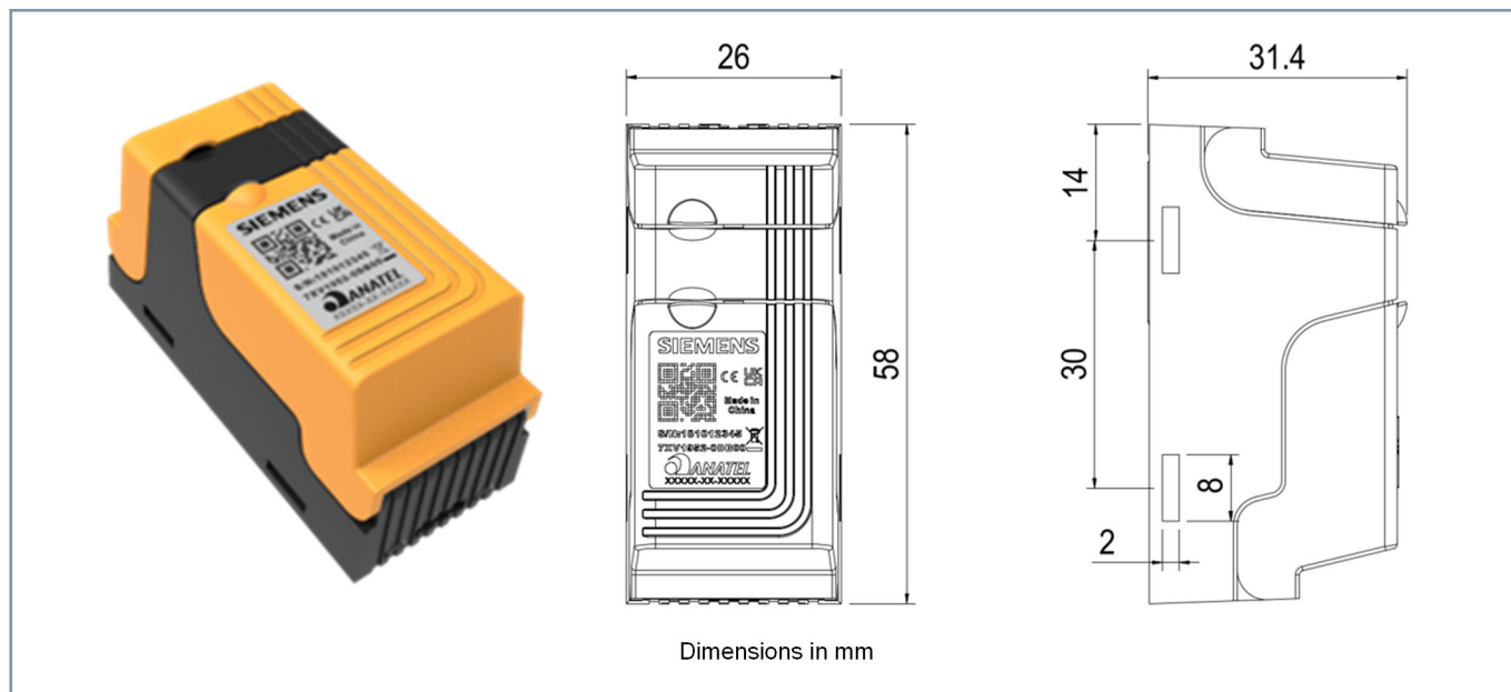
Figure 4.2/4 Wireless Temperature and Humidity Sensor
