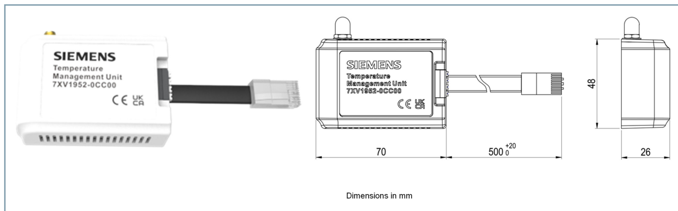
Figure 4.2/5 Temperature Management Unit
