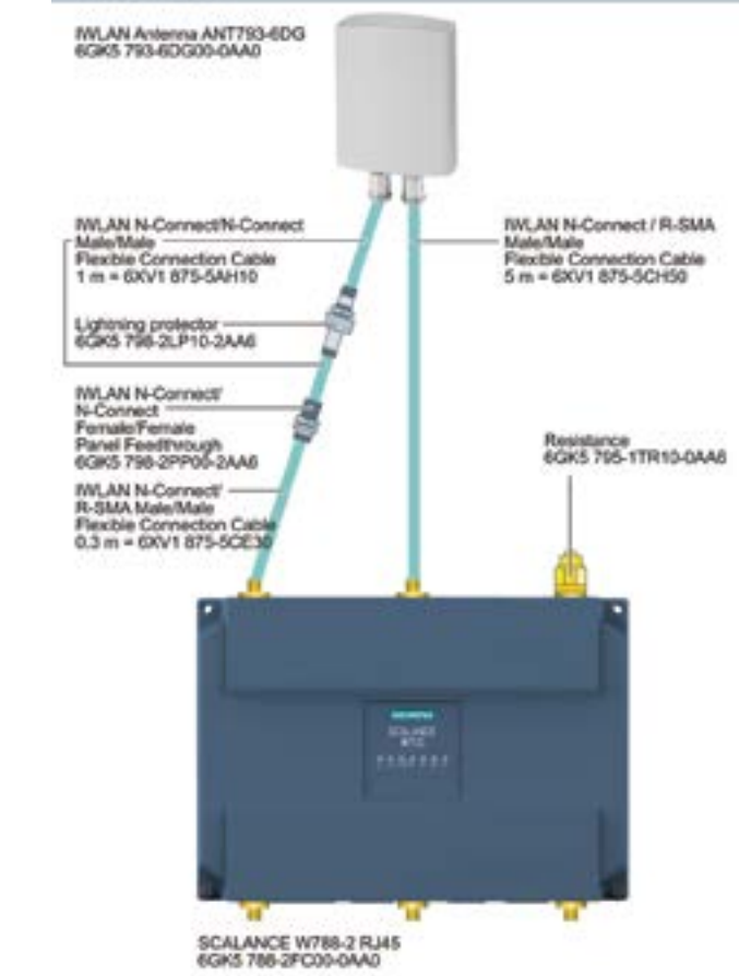
Dual Start antenna ANT793-6DG connected to SCALANCE W788-2 RJ45 with R-SMA ports
