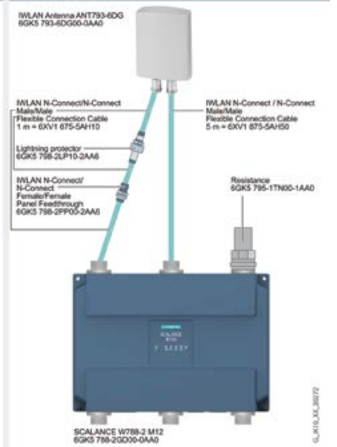
Dual Start antenna ANT793-6DG connected to SCALANCE W788-2 M12 with N-Connect ports
