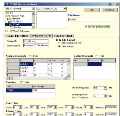
Abbildung 3: COMTRADE-Export (Windows®)
