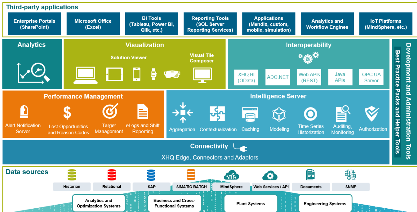
Figure 6. Generalized architecture - most XHQ software is in the middle tier
