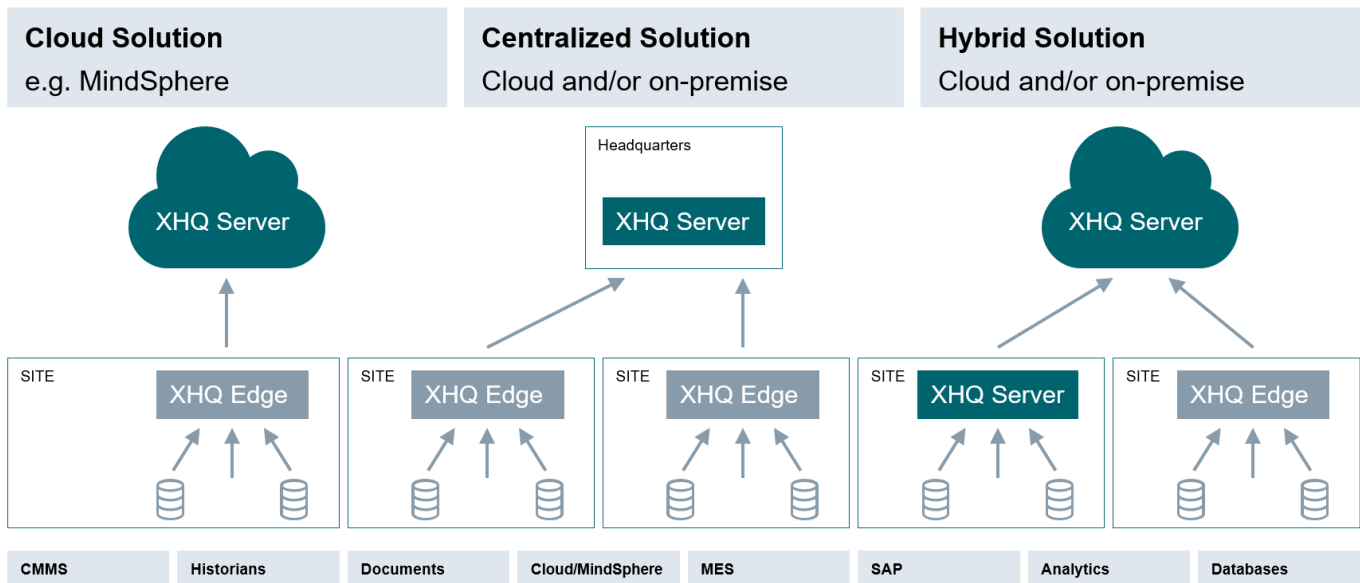
Figure 7. Examples of XHQ Edge usage for site to remote site or site to cloud
