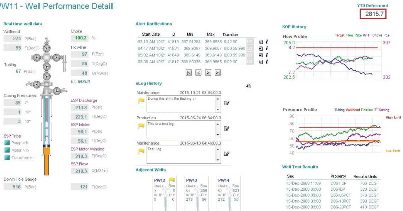
Figure 5. Performance Management adds alerts, logs, and target capabilities
