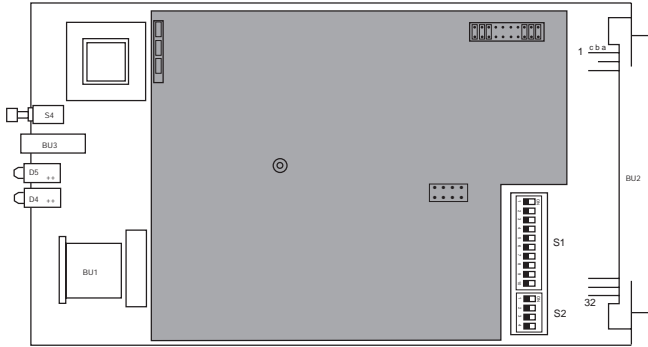
Fig. 6.6: LGM 28.8D1 with DBU Board
