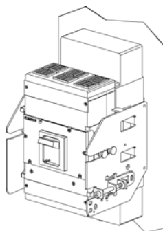
Withdrawable version with front busbar connections
