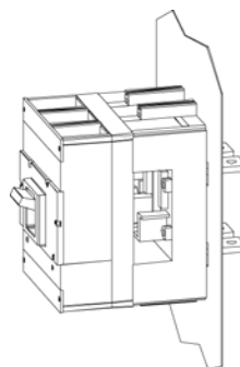
Plug-in base with rear flat busbar terminals
