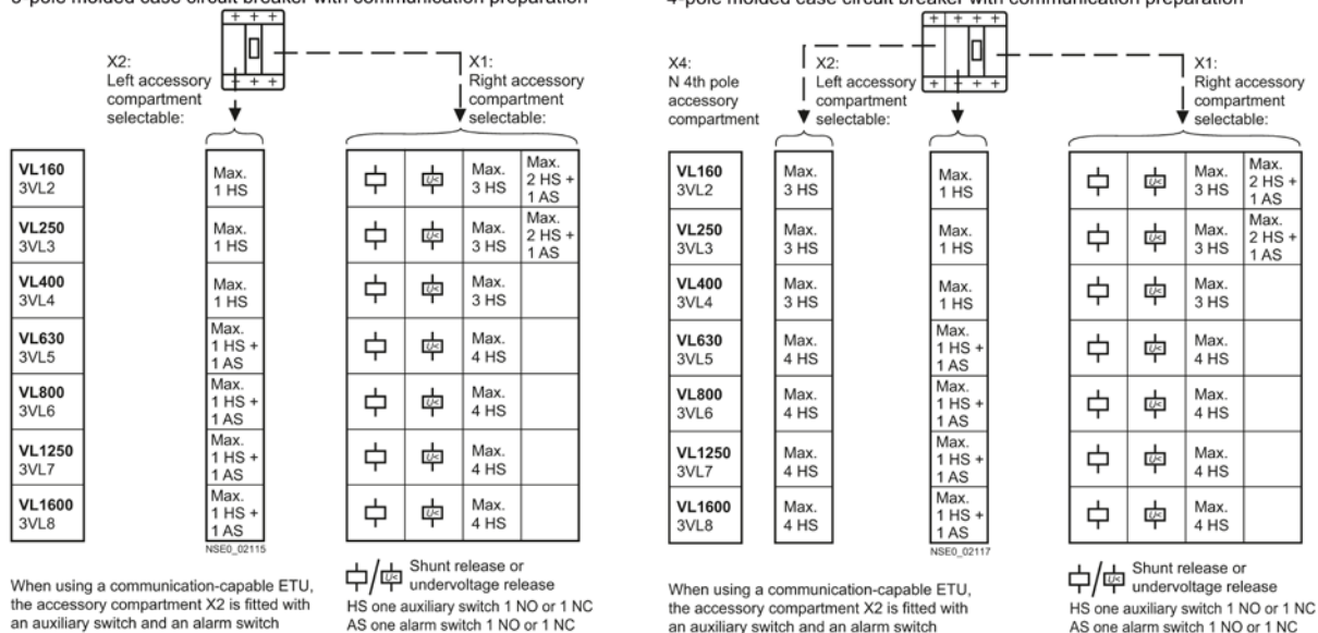
Figure 4-9 Possible complements for the insulated accessory compartments
