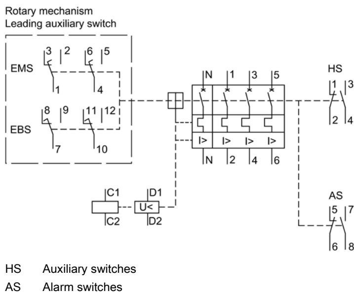
Figure 13-1 Connection diagram for 3- and 4-pole VL160X-VL630 molded case circuit breakers for system protection with thermal-magnetic overcurrent releases
