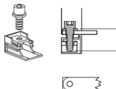
Terminals with screw connection
