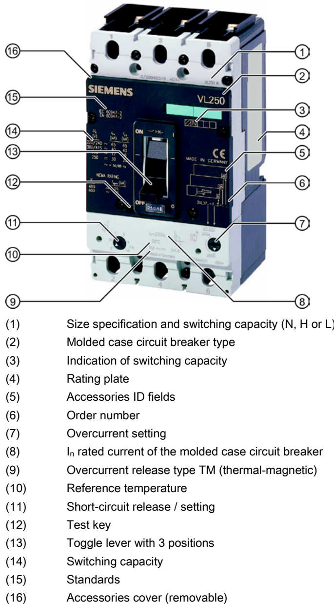
Figure 3-1 3VL molded case circuit breakers - labeling and operator controls
