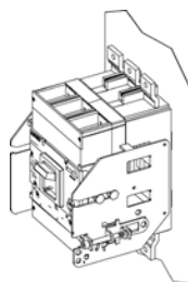
Connected position
