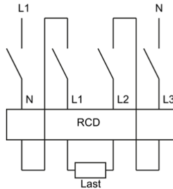
Figure 4-4 4-pole RCD
