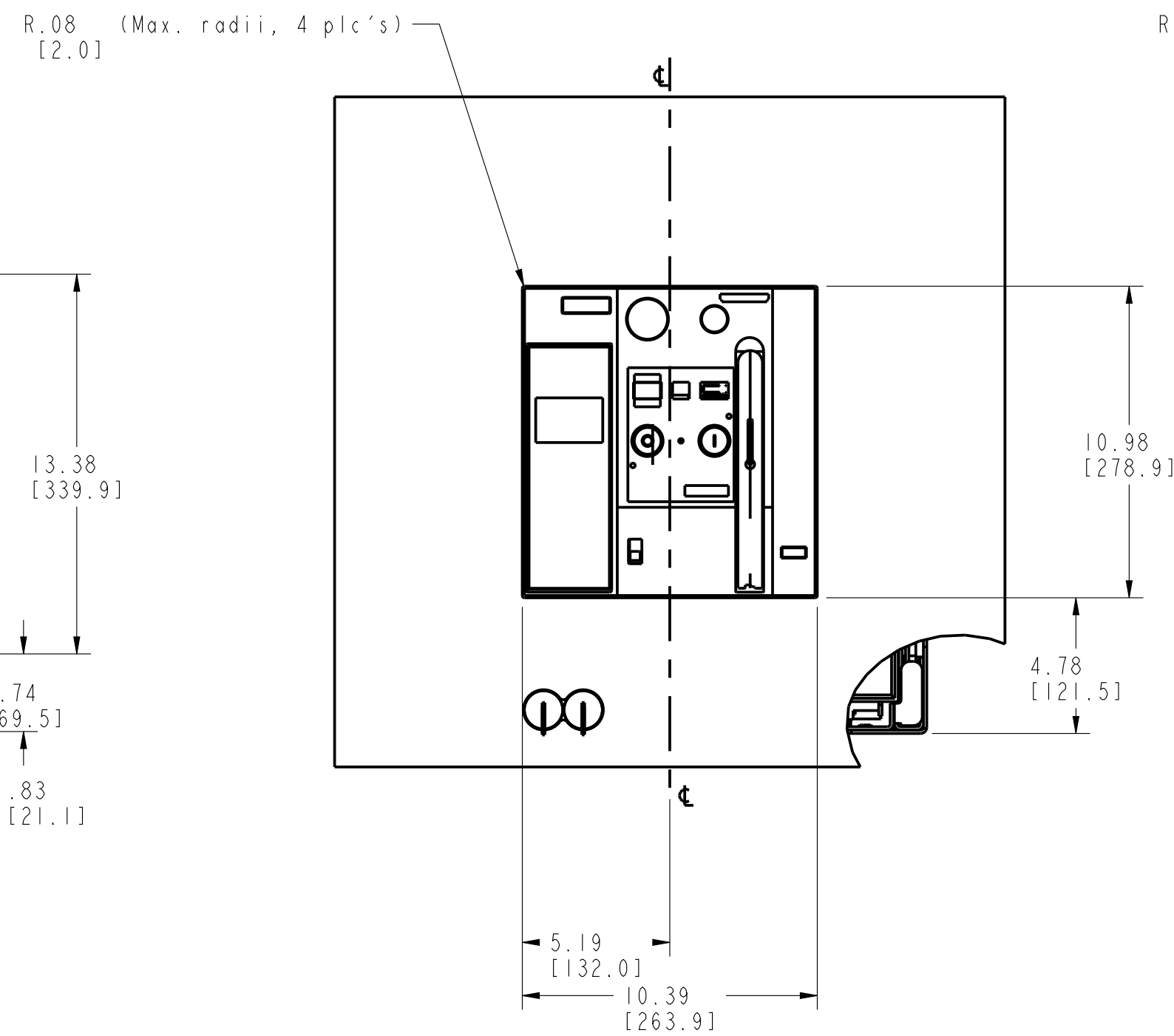
Door cut-out (Middle escutcheon visible)
