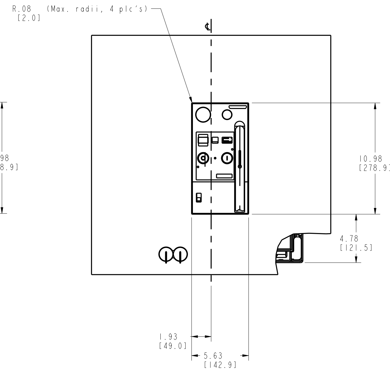
Minimal door cut-out (Only center escutcheon visible)
