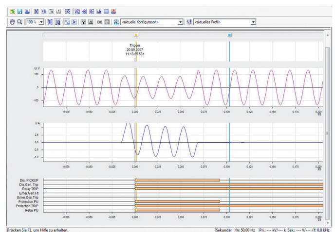
Fault display with diagnostic software Sigra 4
