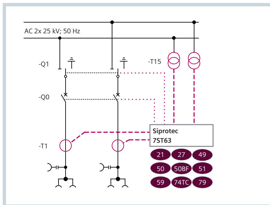
Typical configuration of an AC contact line feeder in the autotransformer system with a numerical overhead contact line control and protection relay (contains optional functions)
