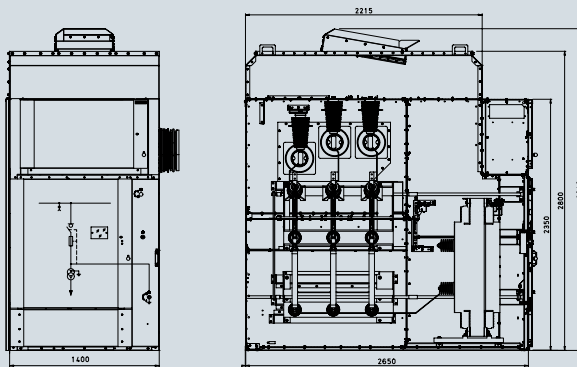
Auxiliary transformer panel
