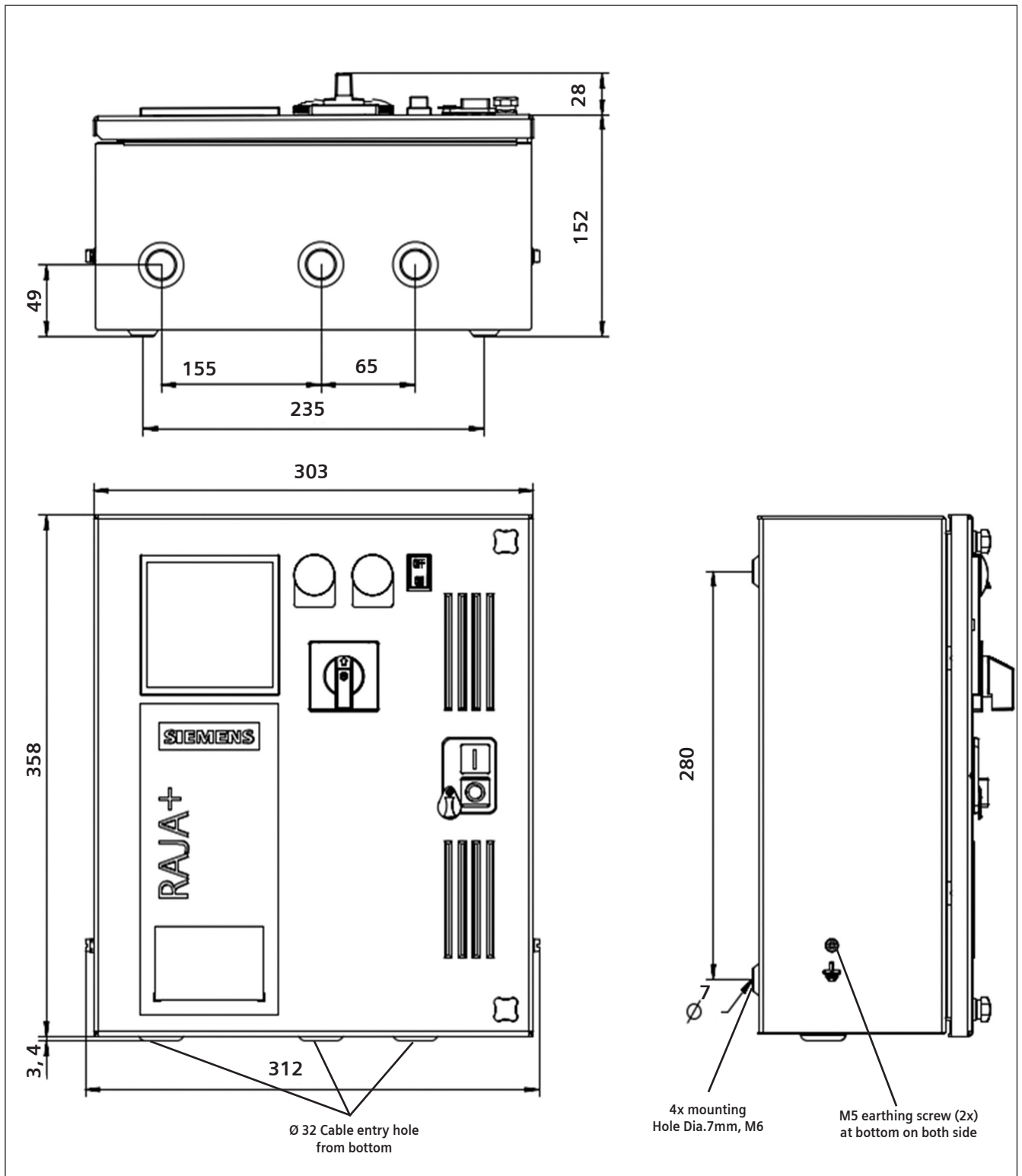
Fig. 5: Dimensional Drawing
