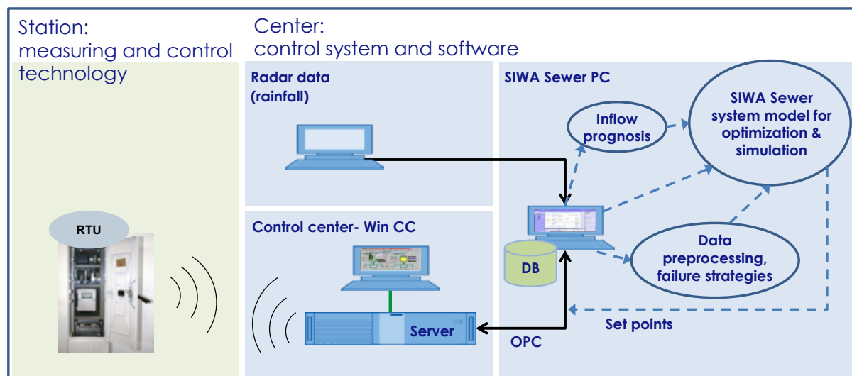
Since 2016, the Erftverband has integrated radar data with inflow modelling and plant control in its sewer network in Kenten
