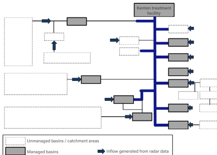
Schematic of the sewer network with managed basins and transfer points for the generated inflows
