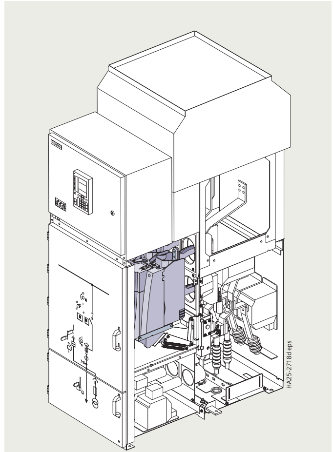
Vacuum circuit-breaker
