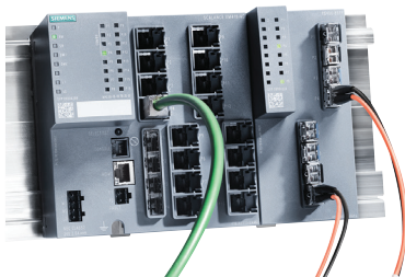
SCALANCE XM416-4C + PE400-8SFP
