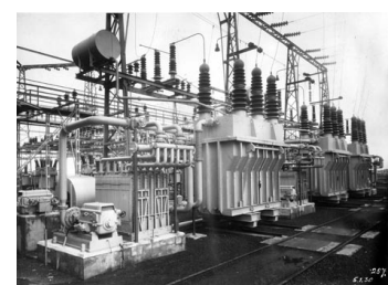
Outdoor transformer station, Inchicore near Dublin, 1930
