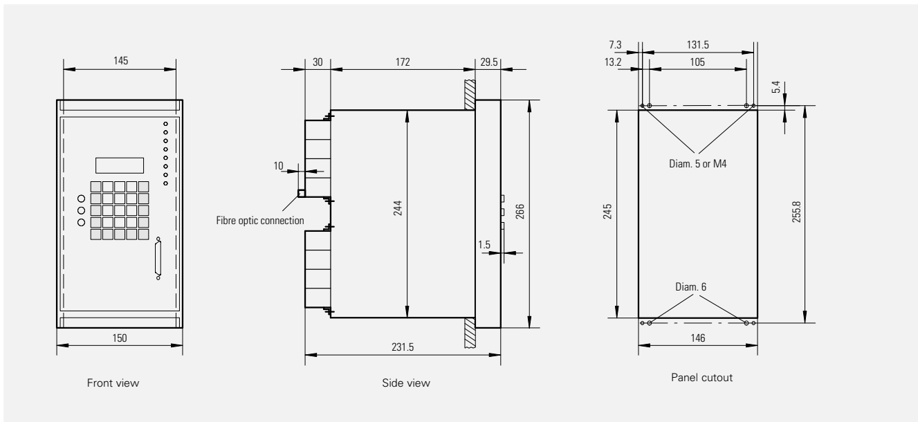
Fig. 4 7SV512 with housing 7XP2030-2 (for panel flush mounting or cubicle mounting)
