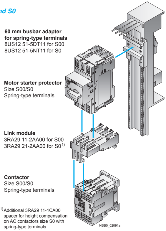
Right: 3RA21 motor starter for direct-on-line starting with busbar adapters with spring-type connection
