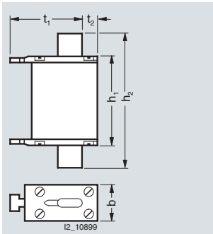
Size 4 (IEC design)
