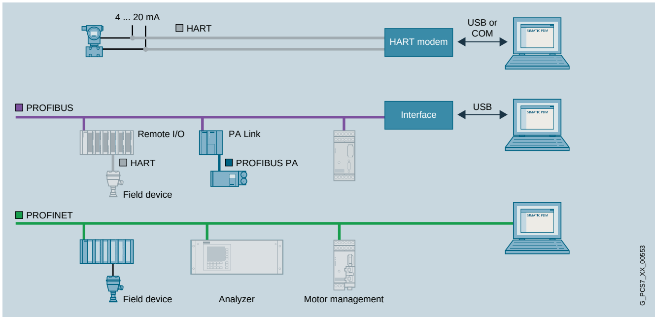
Possible connections of a single point station
