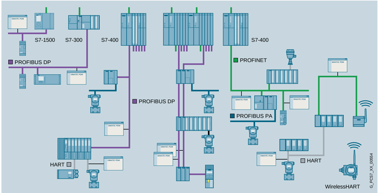
Possible connections for a local service and parameter assignment station
